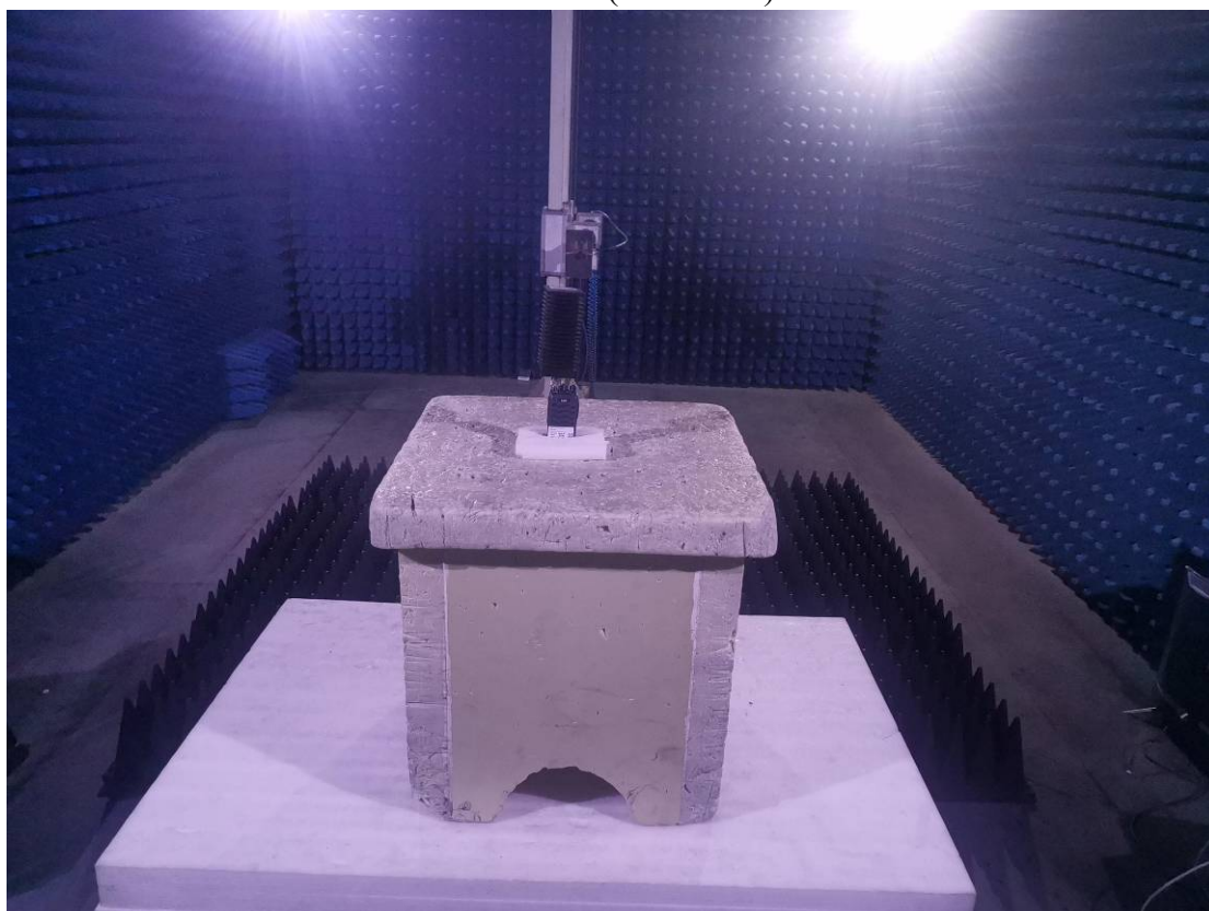
Photo of Radiated Emission Measurement (Above 1G)
