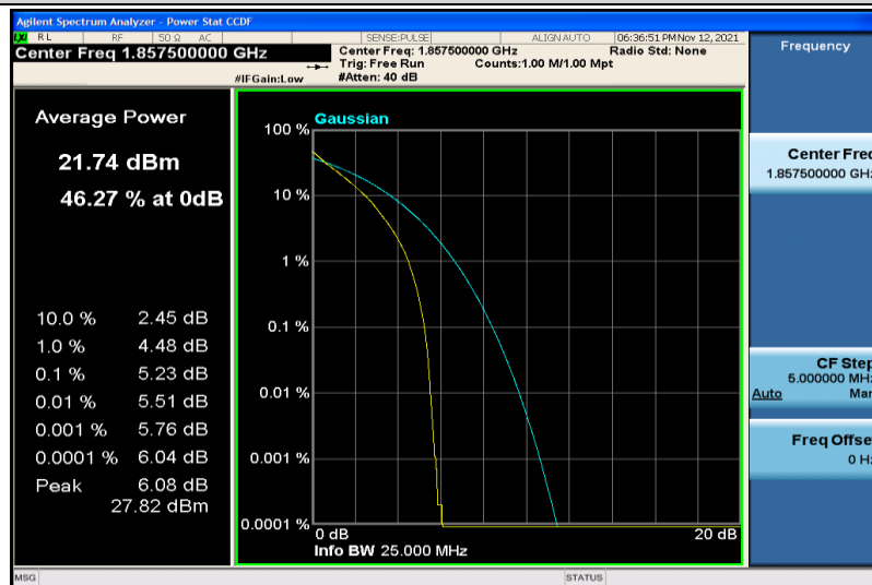
Band2-15MHz-QPSK-18675-5RB#0
