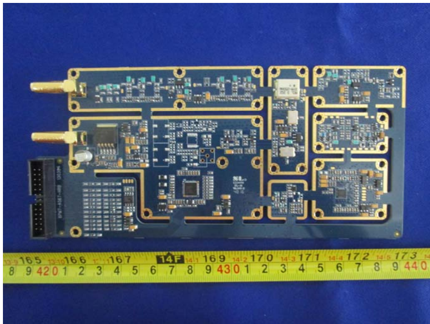
EUT –TX Board Top View
