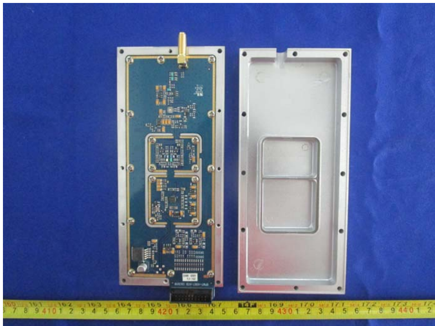
EUT – RX Board Cover Off View
