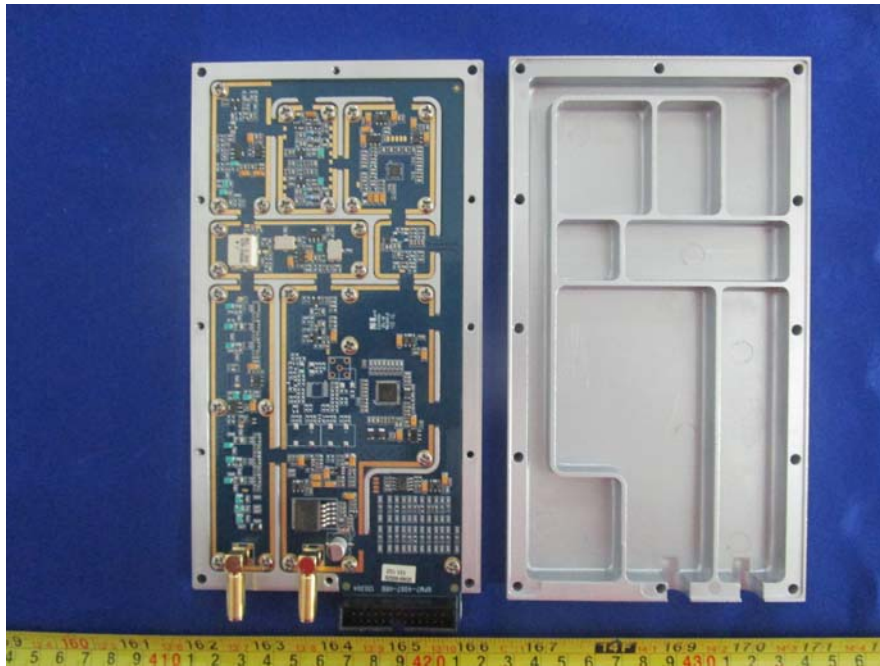
EUT – TX Board Cover Off View
