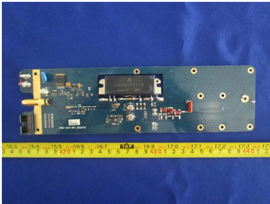
EUT – PA Board Top Unshielded View
