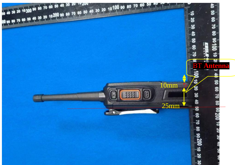
Antenna position
