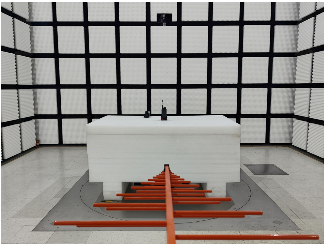
Radiated Emission Below 1GHz View For model: DP585
