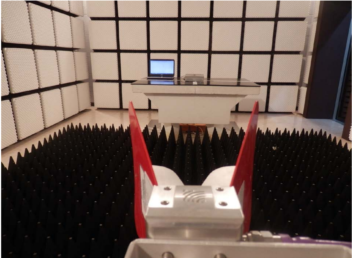
Photograph 2: Test Setup for Above 1 GHz
