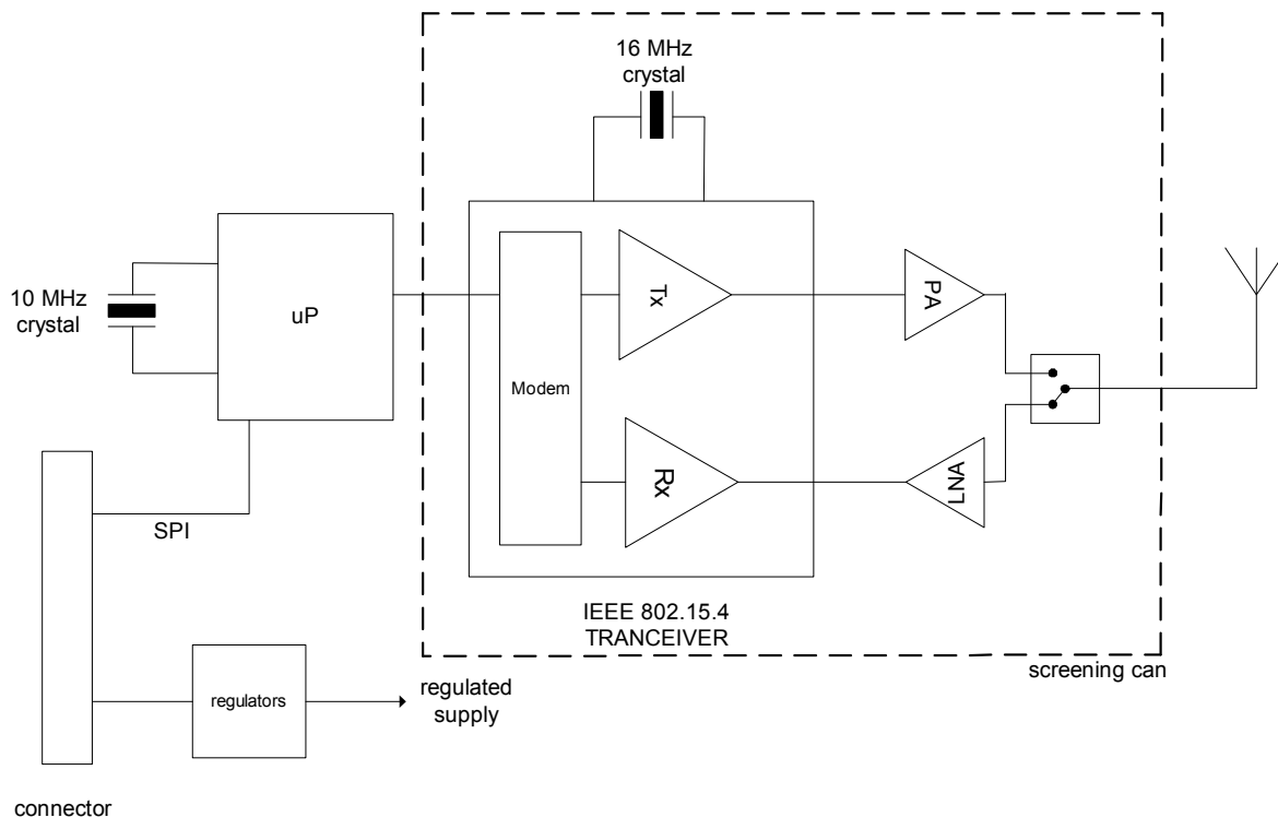
Figure 1. S10011 Block Diagram
