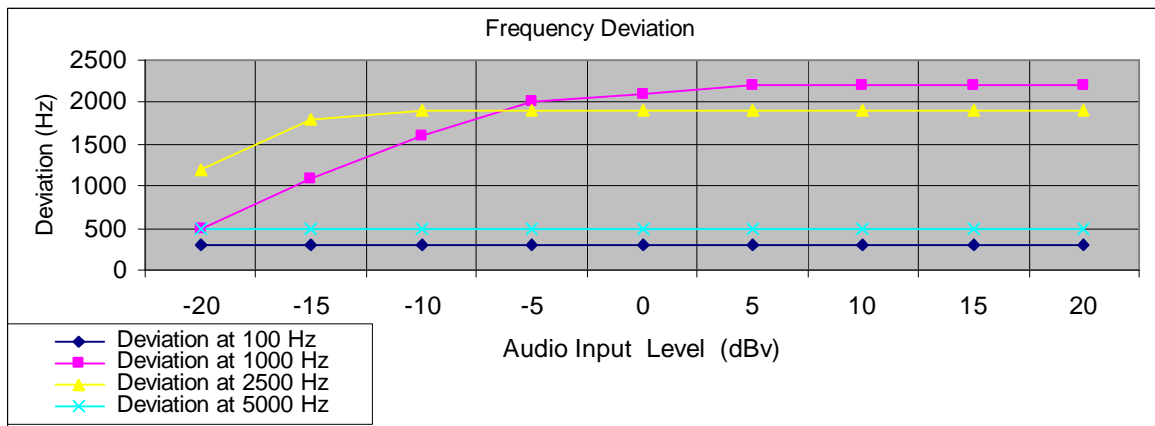
Figure 2 Deviation Characteristics.
