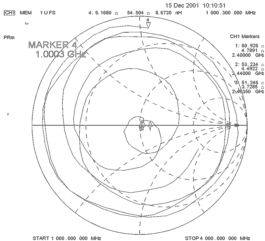
Fig 3. Smith Chart
