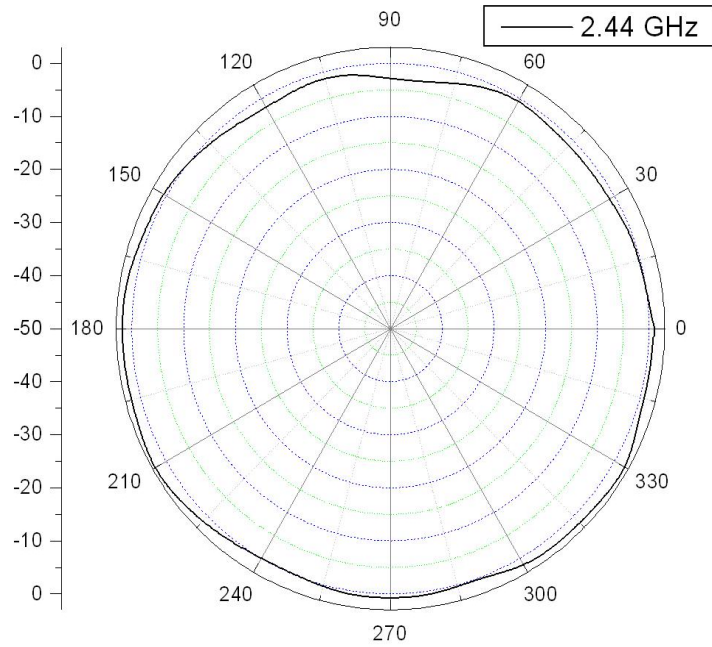
Azimuth Pattern
