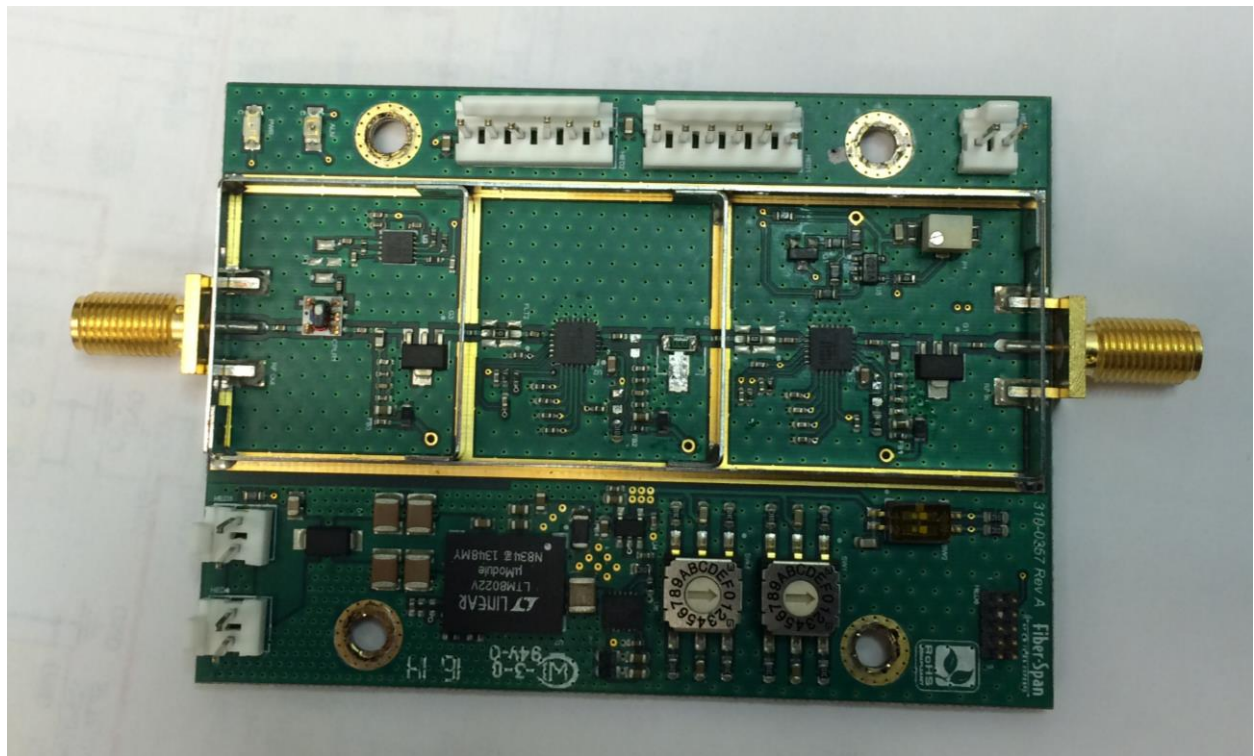
LNA Board
