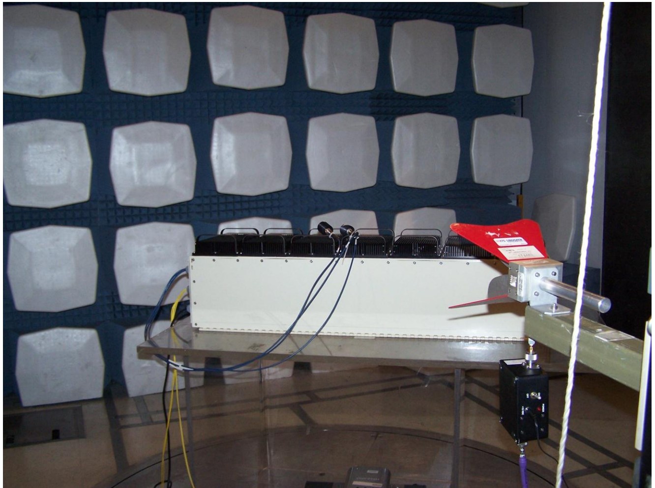
Photograph 5. Radiated Spurious, Test Setup, Above 1 GHz
