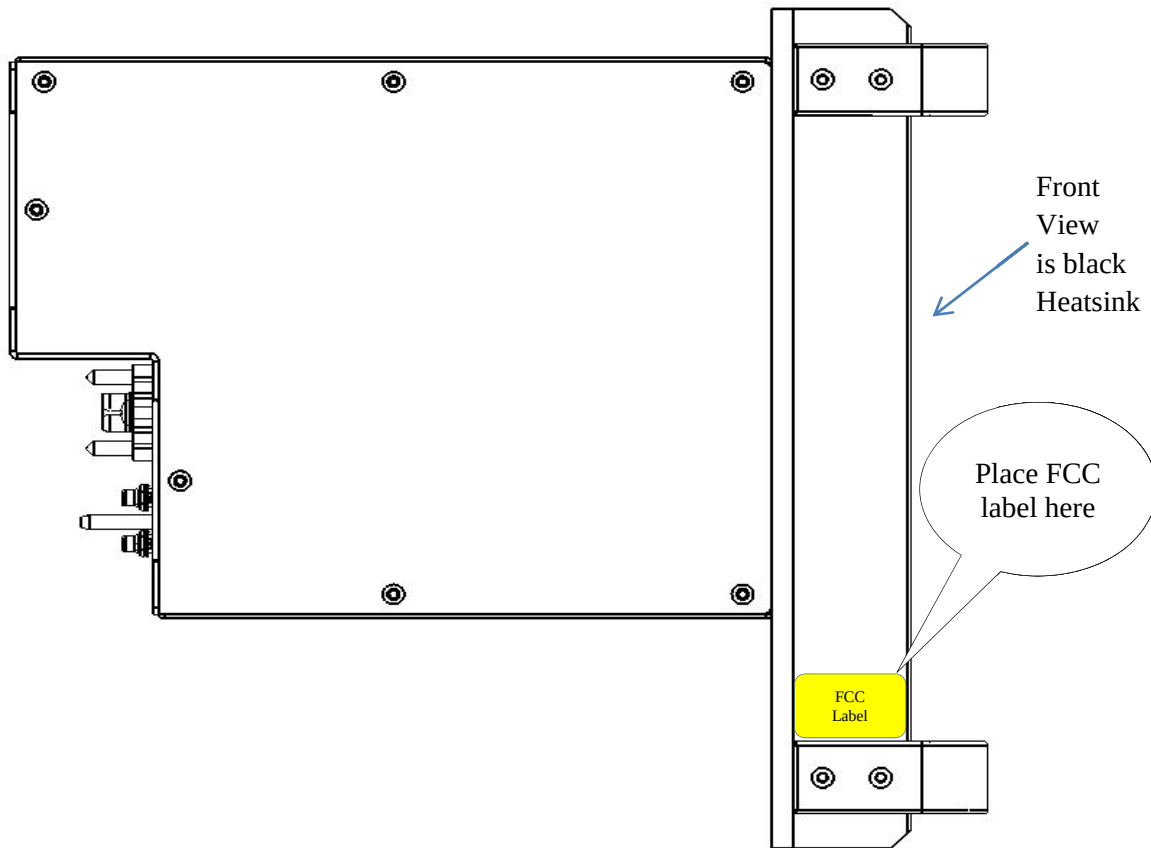
LEFT VIEW
