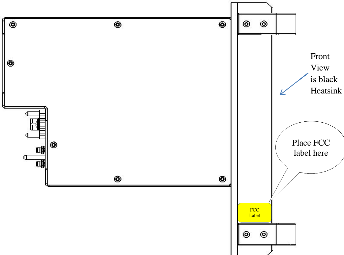
LEFT VIEW
