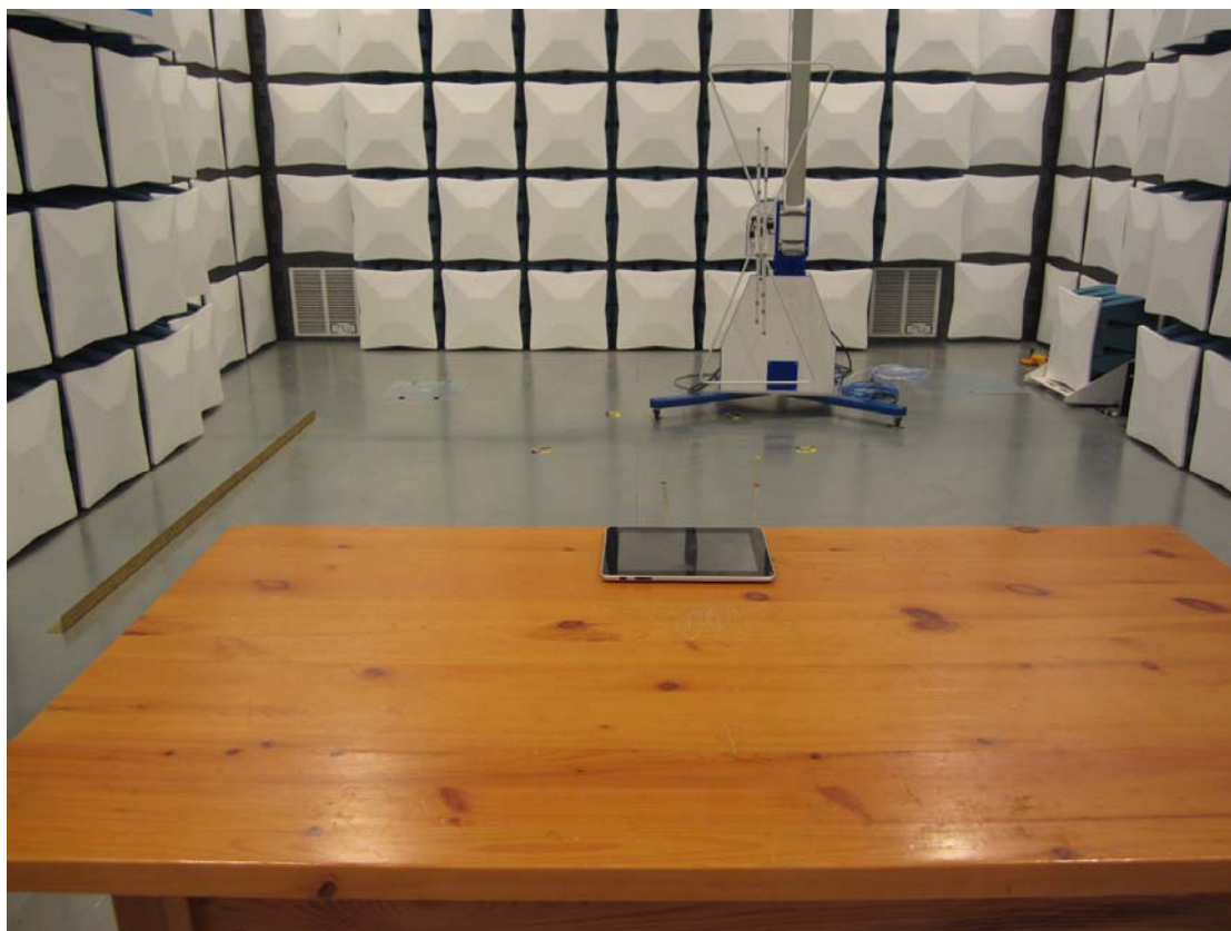
Radiated Emission Test Setup in Chamber
