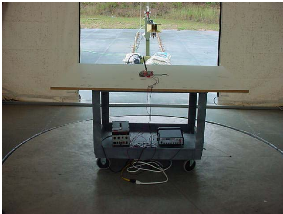
Figure 2: Radiated Emissions – Rear View
