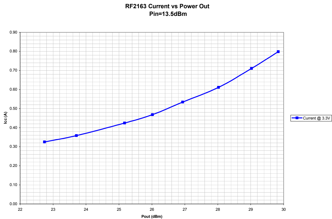
Figure 1: Current vs. Power Out at 3.3 volts at the final amplifier stage
