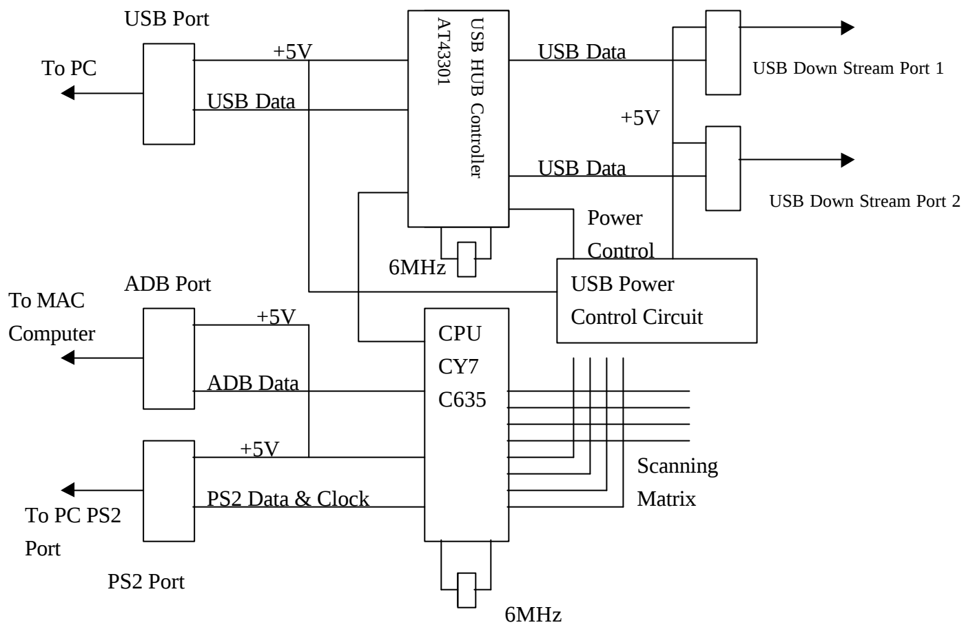
Block Diagram for Keyboard Model Number FK101
