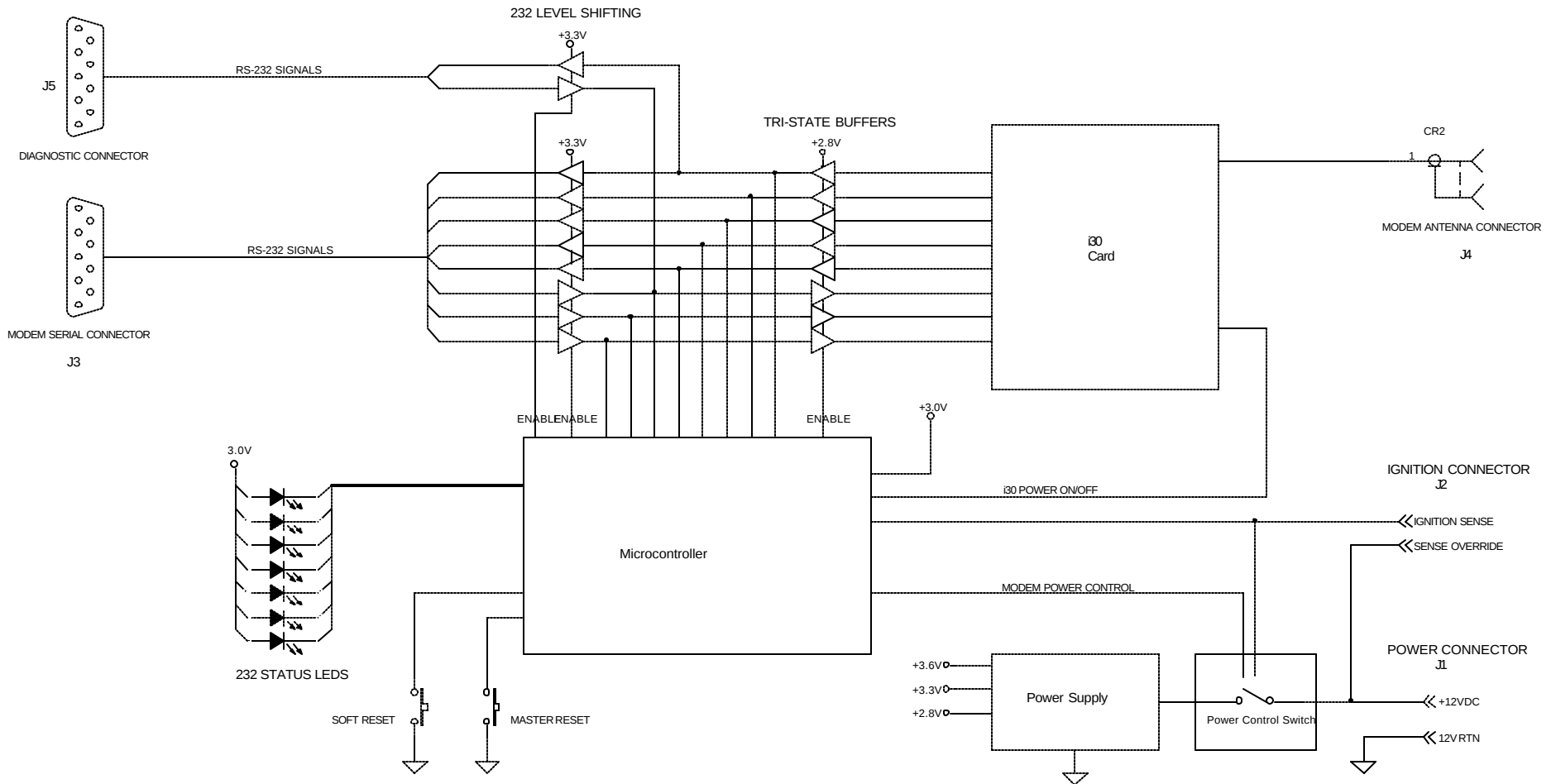
IR1200 Modem Block Diagram
