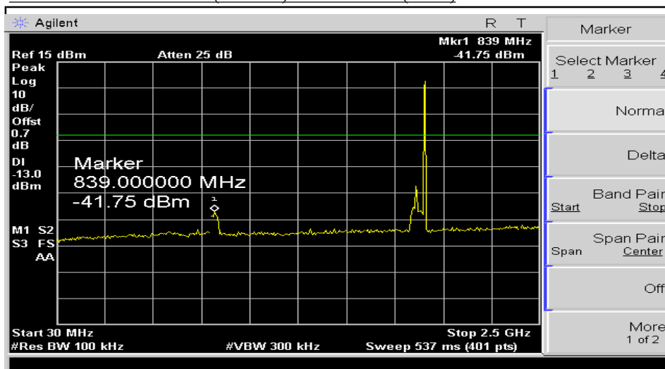
PLOTS OF EMISSION (CDMA) Out of Band (1175)
