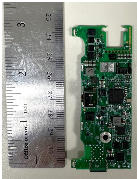
Fig. 2. Charger internal photo PCB – Frontside
