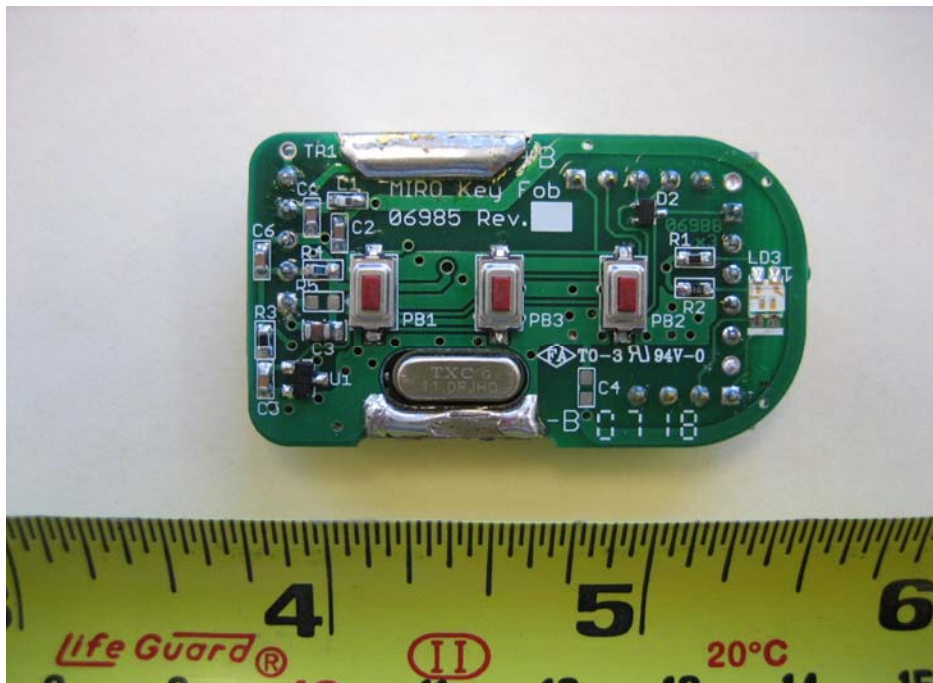
EUT Board Components View
