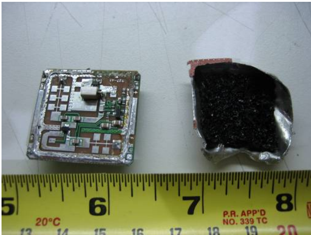
Radio Module Shielding Off View
