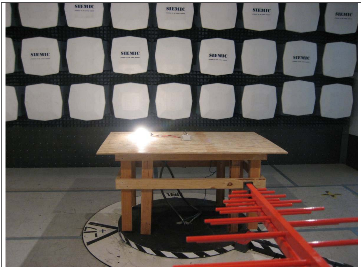
Radiated Emission Test Setup – Front View (<1GHz)
