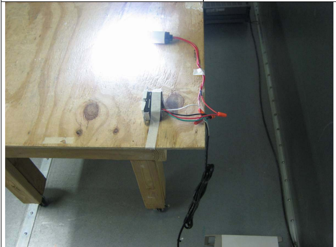
Conducted Emission Test Setup – Rear View
