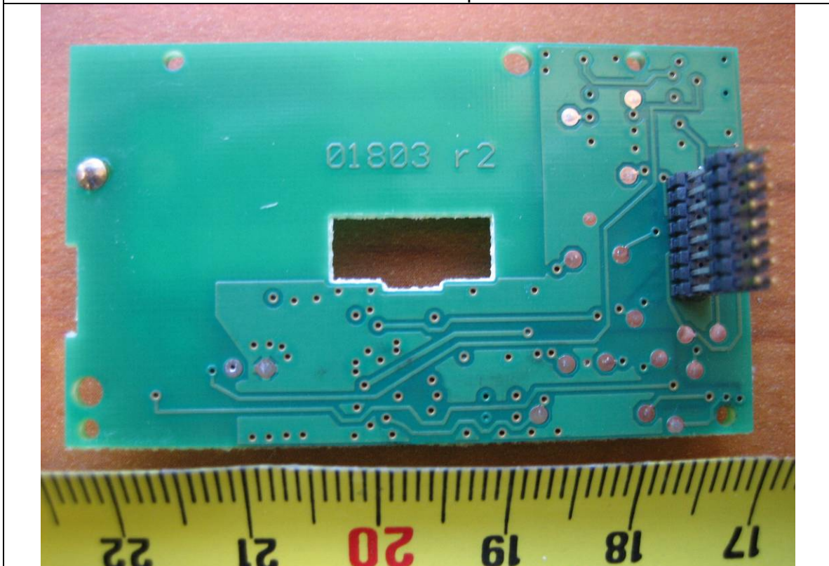
EUT – RF PCBA Solder View
