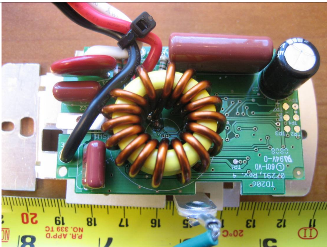
EUT Supply – PCBA Component View 1
