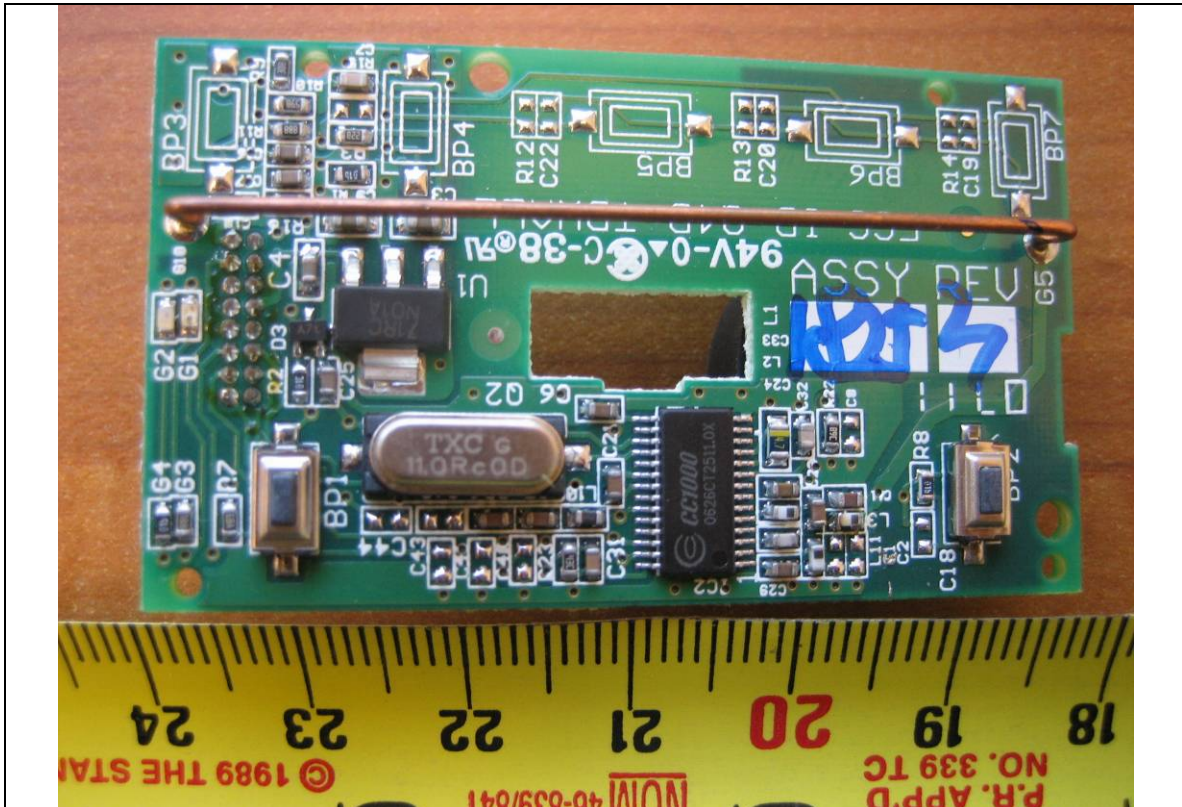
EUT – RF PCBA Component View
