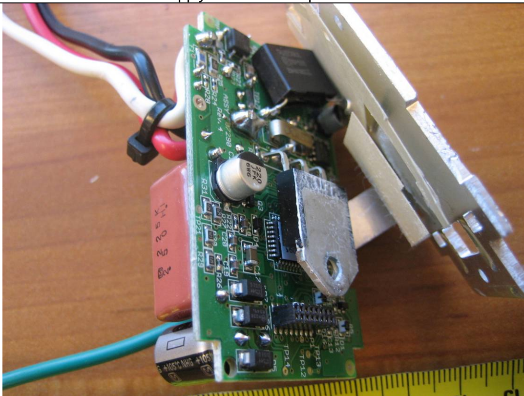
EUT Supply – PCBA Component View 2
