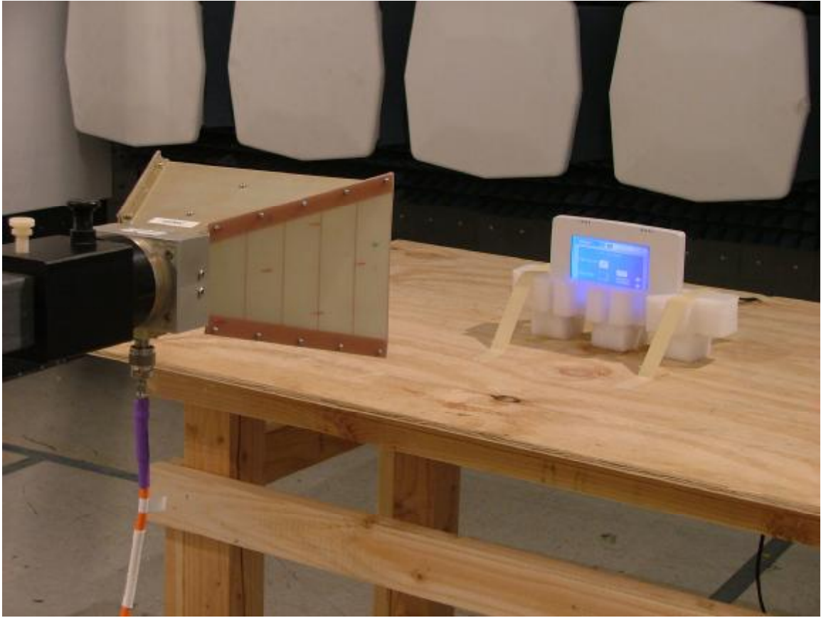
Radiated Emissions > 1GHz
