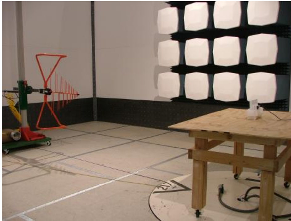
Radiated Emissions < 1GHz
