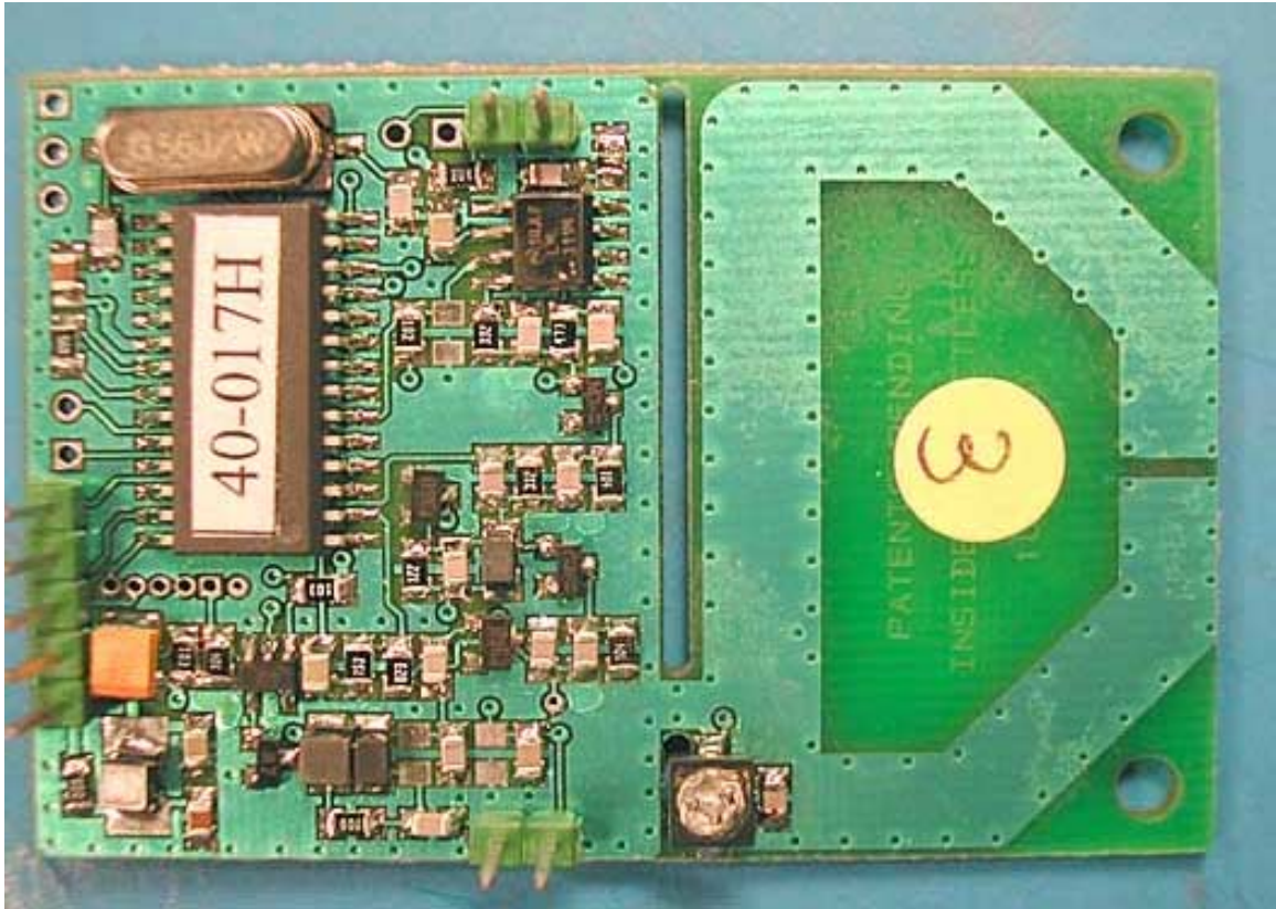
Top with Antenna (on the right)
