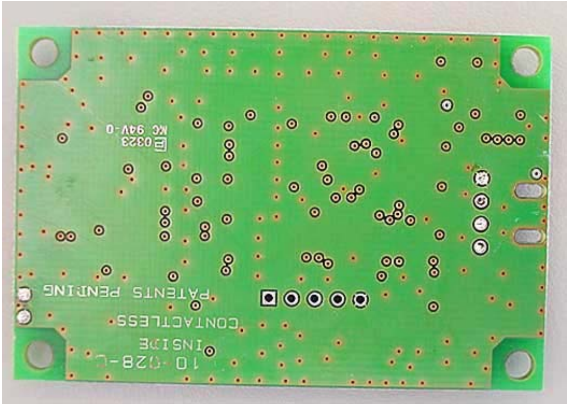
Bottom Main PCB
