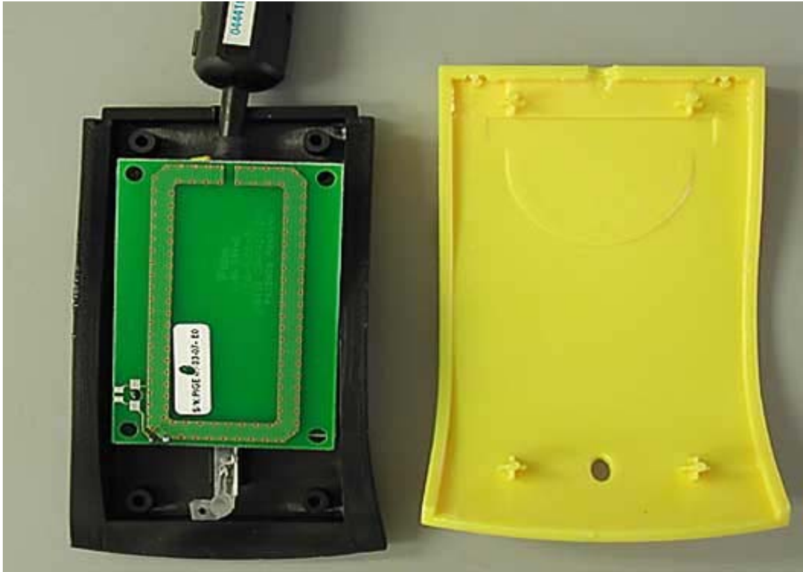
Top Cover Off
