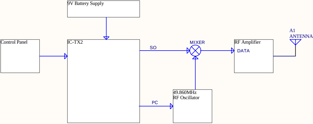
Block diagram
