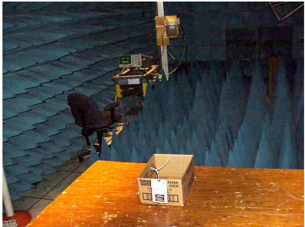
View of Radiated Emissions Prescan 1GHz to 5GHz
