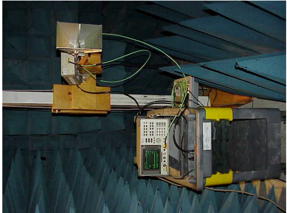
Close up view of 1GHz to 5GHz Radiated Emissions prescan test setup
