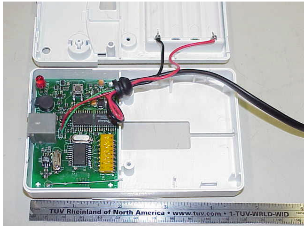
Internal View of Transmitter
