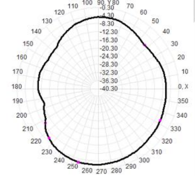
Total(H-XY), Max= -2.59dBi, CirD=9.40
