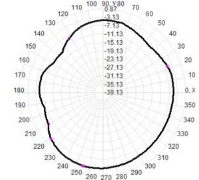
Total(H-XY), Max= -2.78dBi, CirD=9.13
