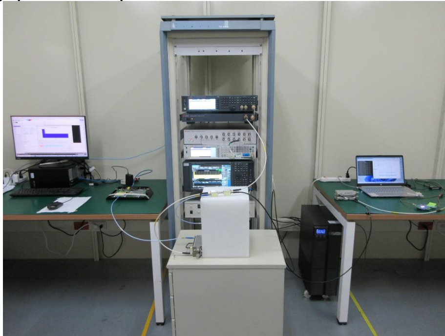
Photograph 9: Test Setup for DFS
