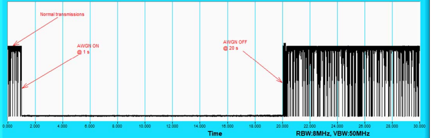
802.11ax (HE160) / CH143(Low Edge)
