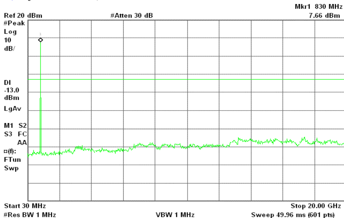
Figure 7-5: Out of Band emission at antenna terminals – GPRS CH Mid
