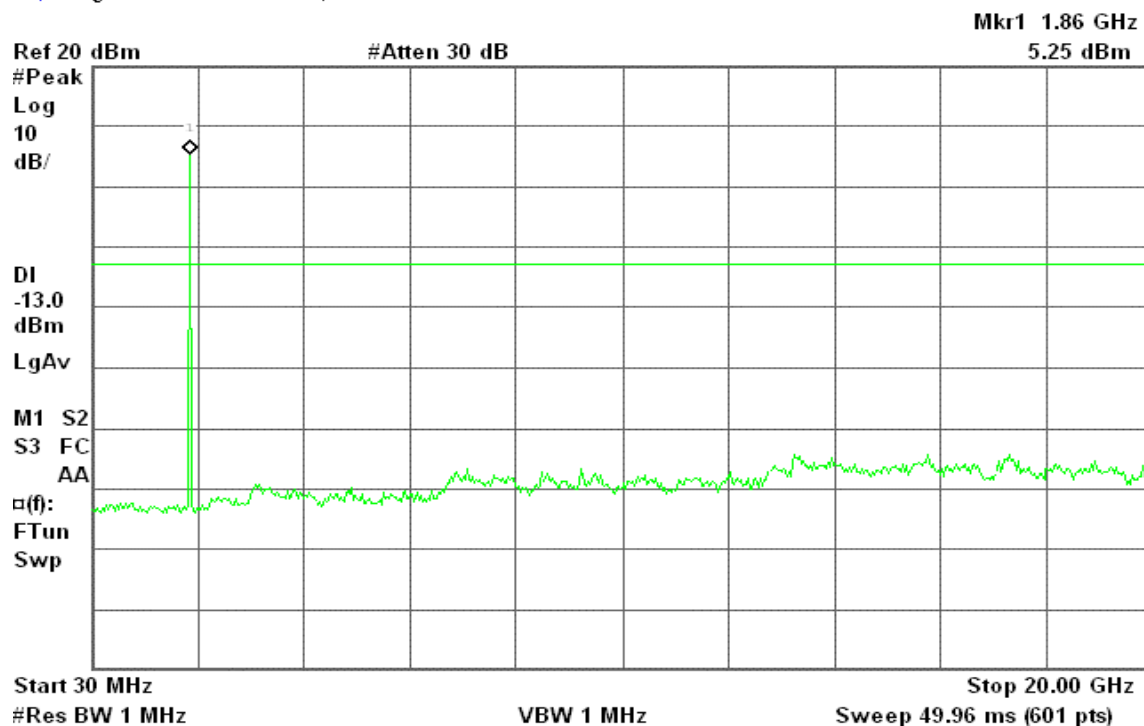
Figure 8-2: Out of Band emission at antenna terminals – GSM CH Mid
