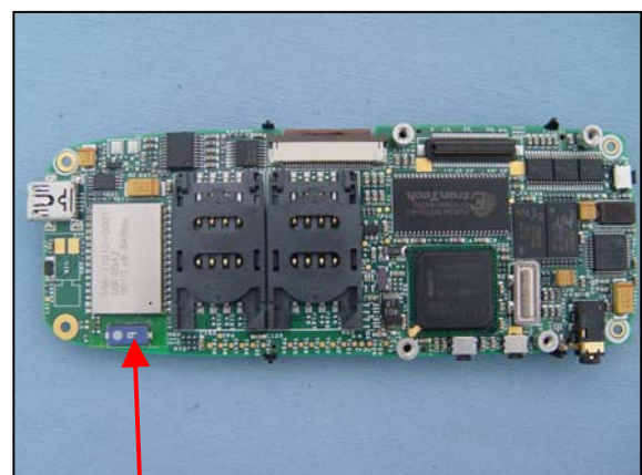
Bluetooth antenna
