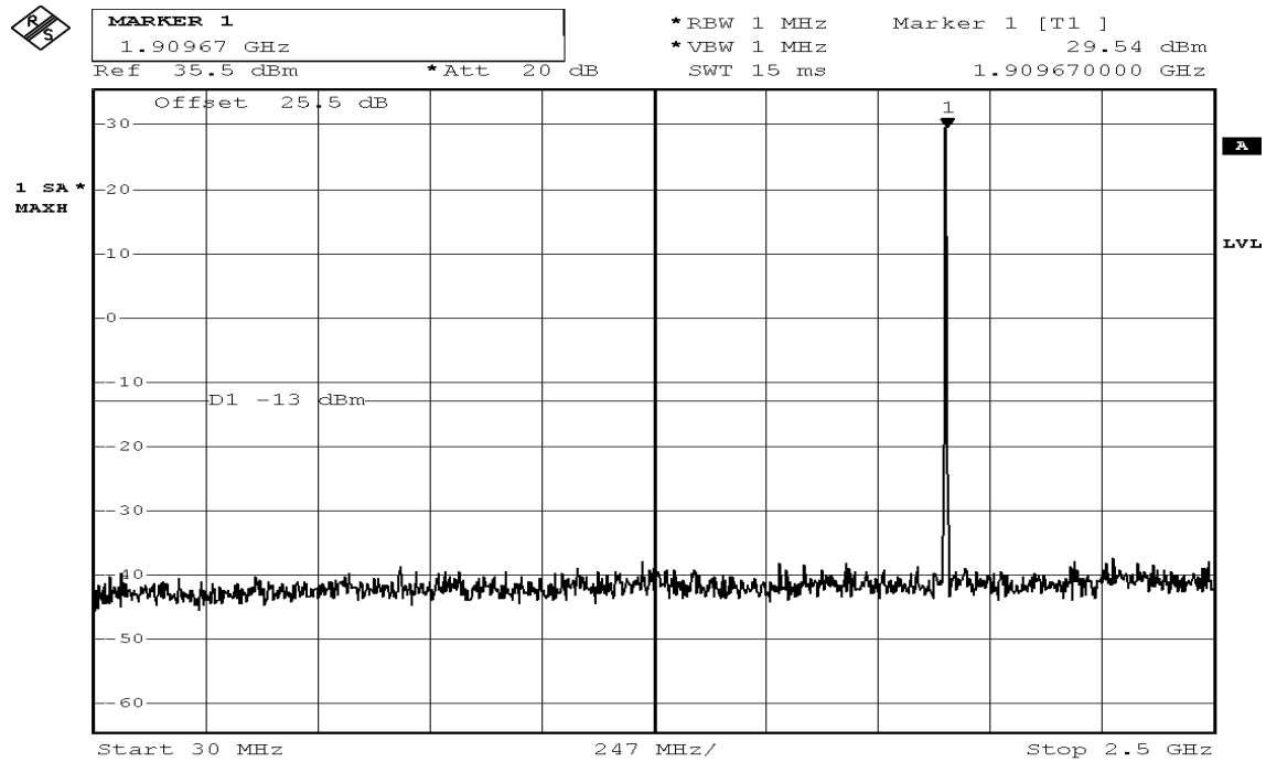
Figure 8-11: Out of Band emission at antenna terminals – GPRS CH High
