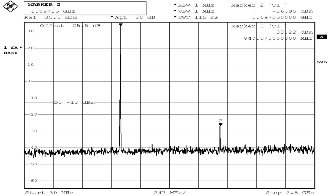
Figure 7-11: Out of Band emission at antenna terminals – GPRS CH High
