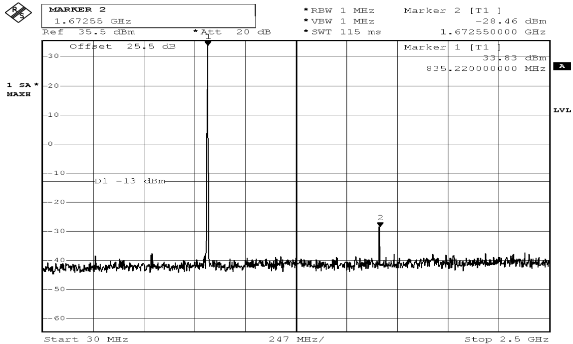
Figure 7-3: Out of Band emission at antenna terminals – GSM CH Mid
