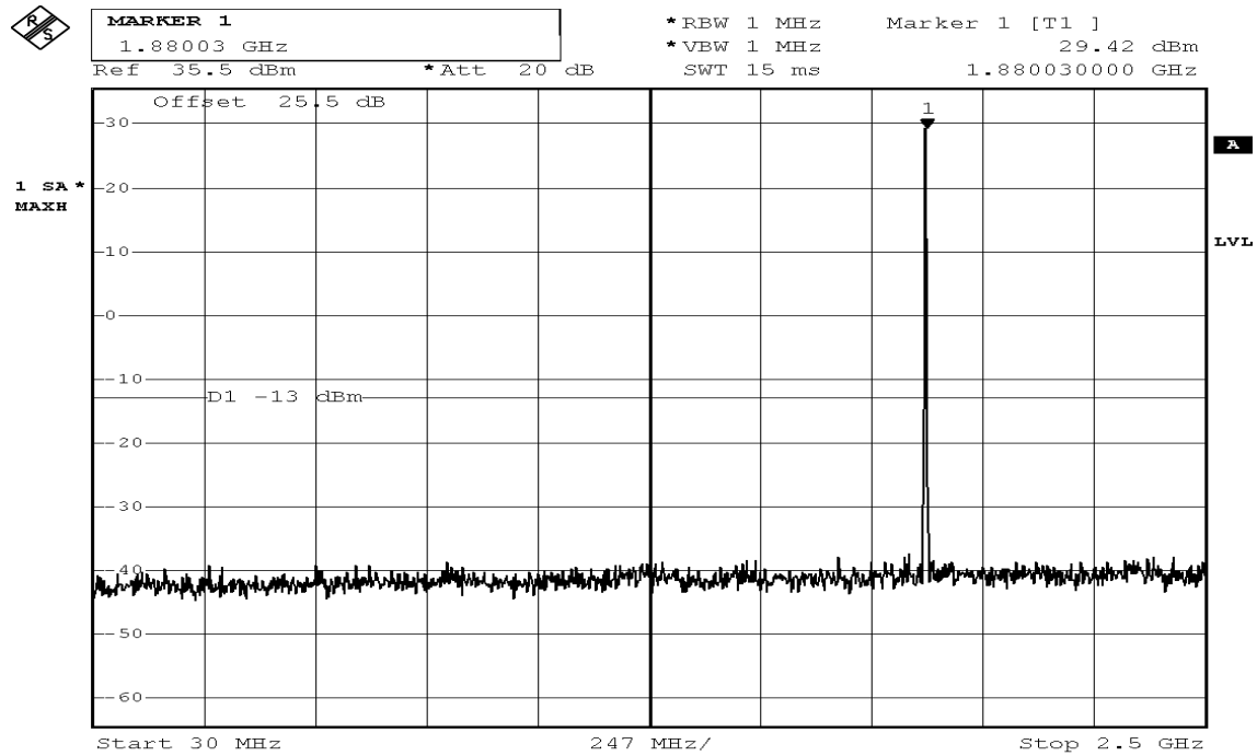
Figure 8-3: Out of Band emission at antenna terminals – GSM CH Mid
