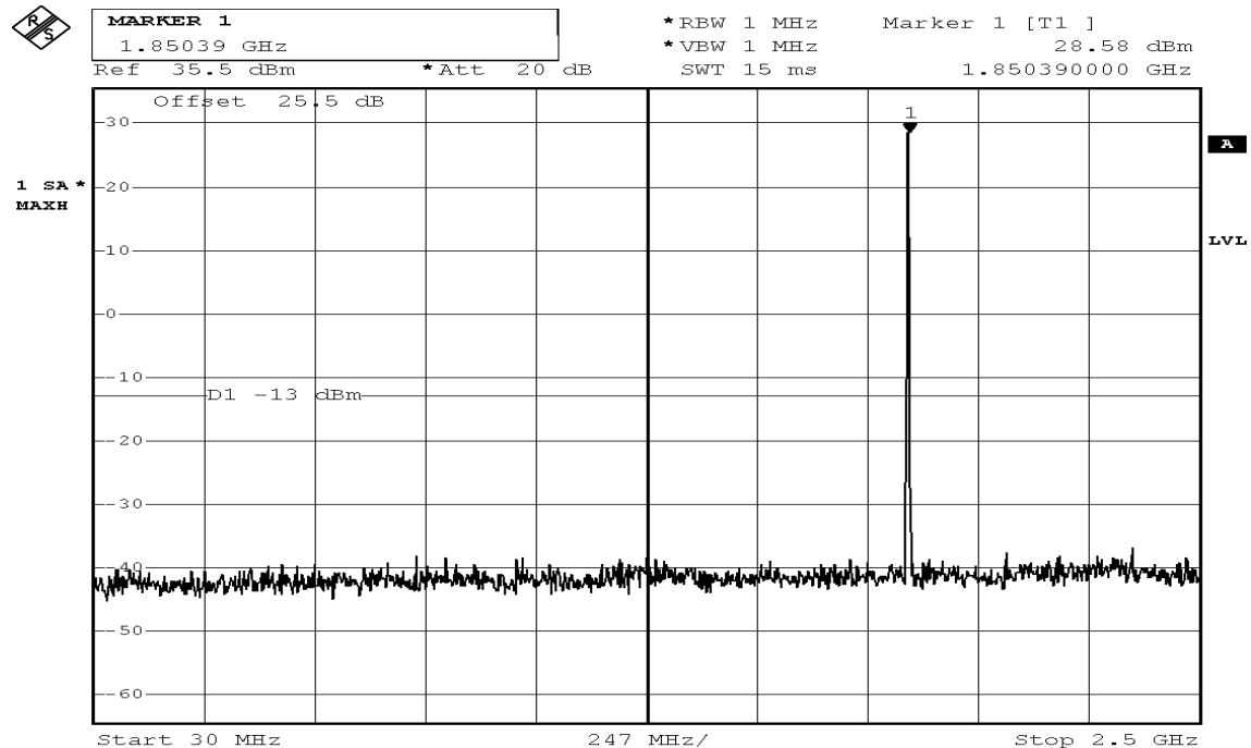
Figure 8-7: Out of Band emission at antenna terminals – GPRS CH Low
