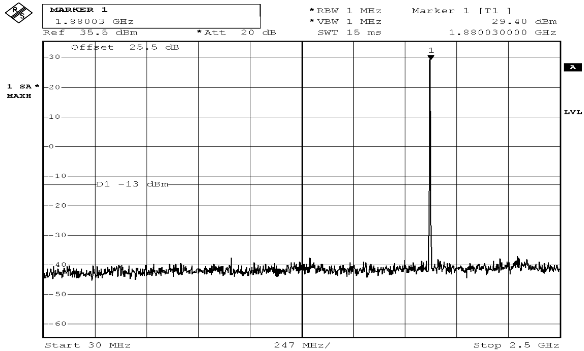
Figure 8-9: Out of Band emission at antenna terminals – GPRS CH Mid
