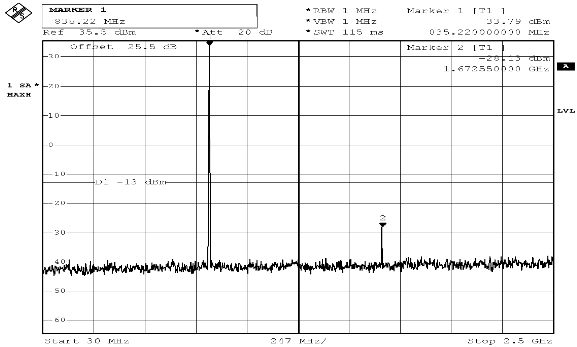
Figure 7-9: Out of Band emission at antenna terminals – GPRS CH Mid
