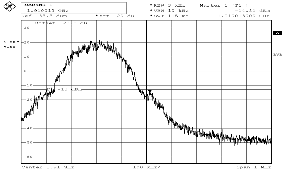
Figure 10-4: Band Edge emissions – GPRS CH High
