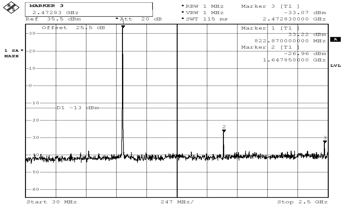
Figure 7-7: Out of Band emission at antenna terminals – GPRS CH Low
