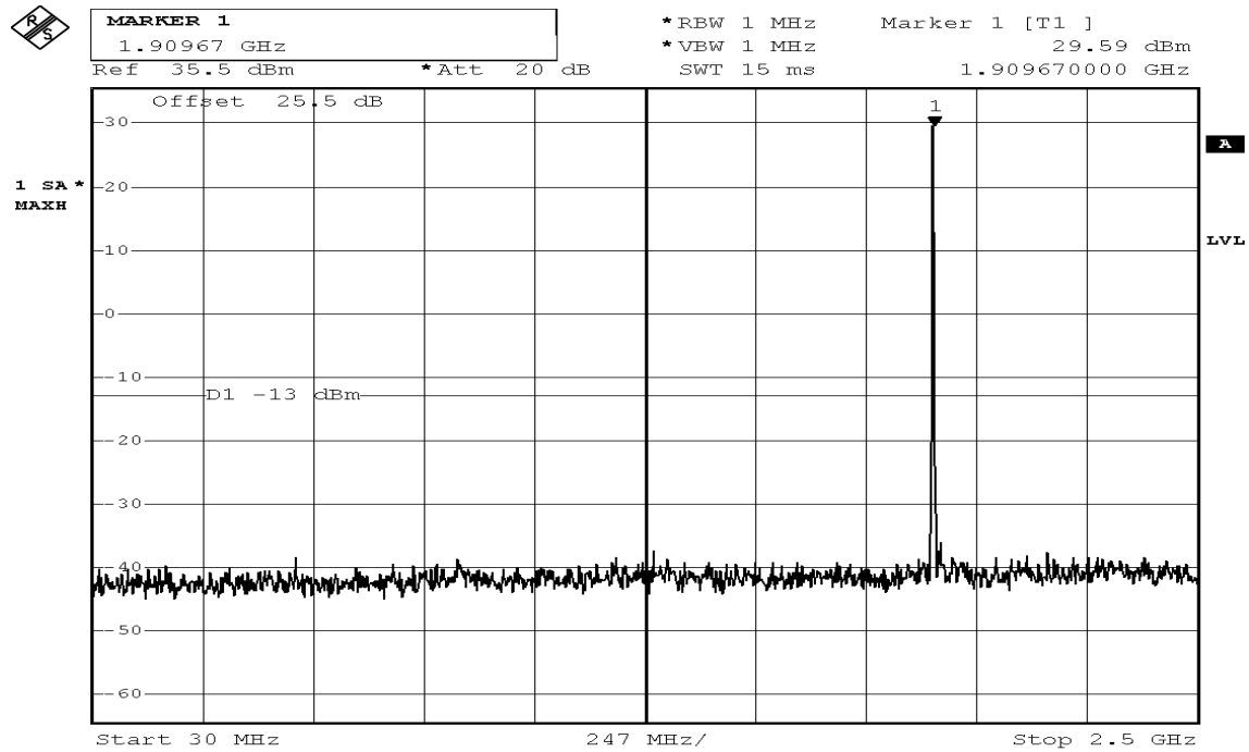
Figure 8-5: Out of Band emission at antenna terminals – GSM CH High
