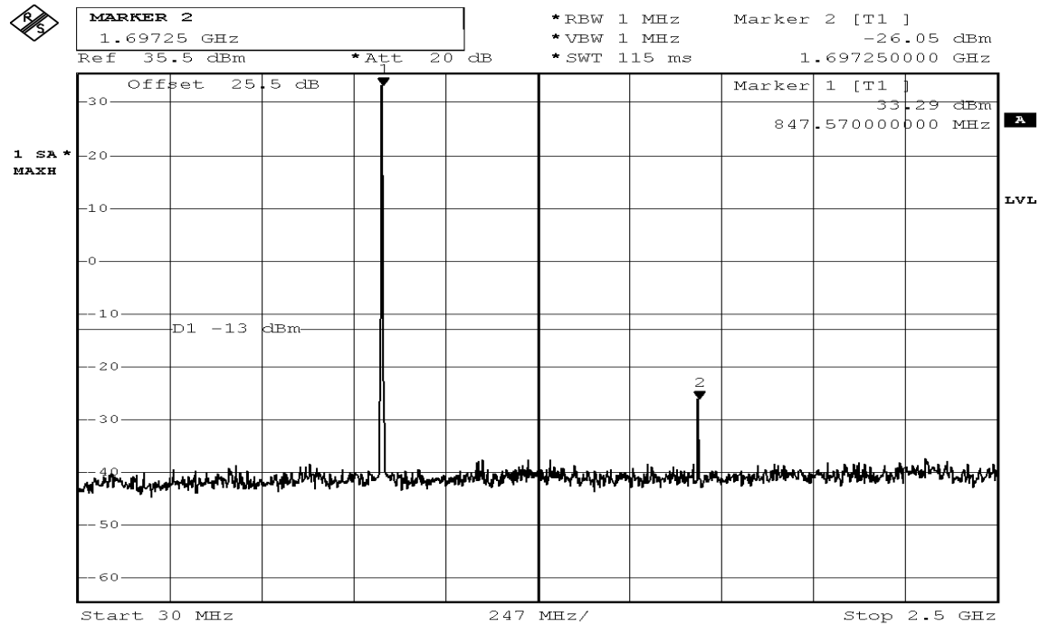
Figure 7-5: Out of Band emission at antenna terminals – GSM CH High
