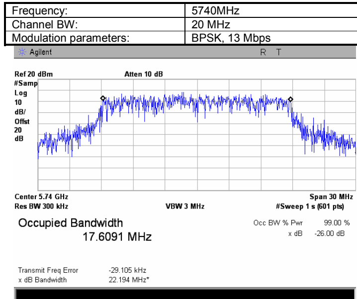
Plot 8.1.10 The 99%power bandwidth test result at low frequency
