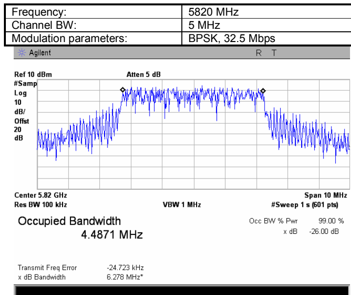
Plot 8.1.32 The 99%power bandwidth test result at low frequency
