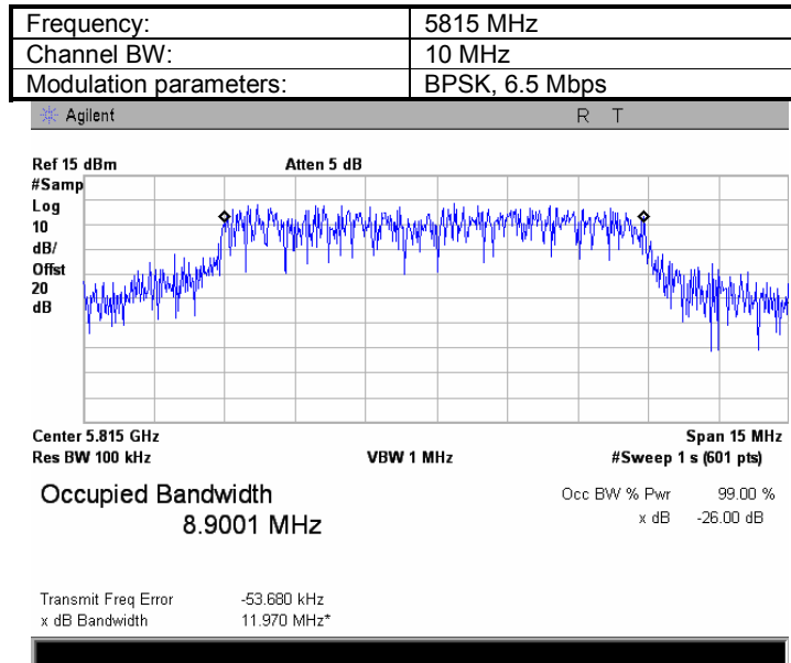
Plot 8.1.24 The 99%power bandwidth test result at low frequency
