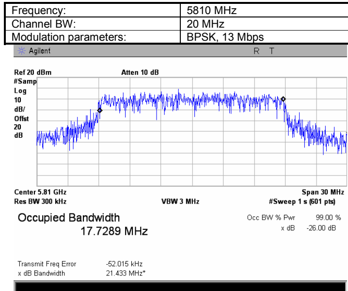
Plot 8.1.14 The 99%power bandwidth test result at low frequency
