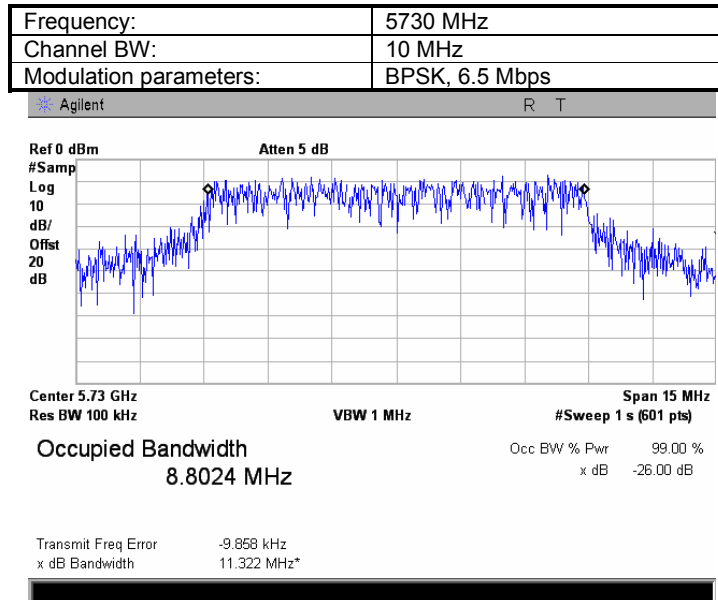
Plot 8.1.18 The 99%power bandwidth test result at low frequency
