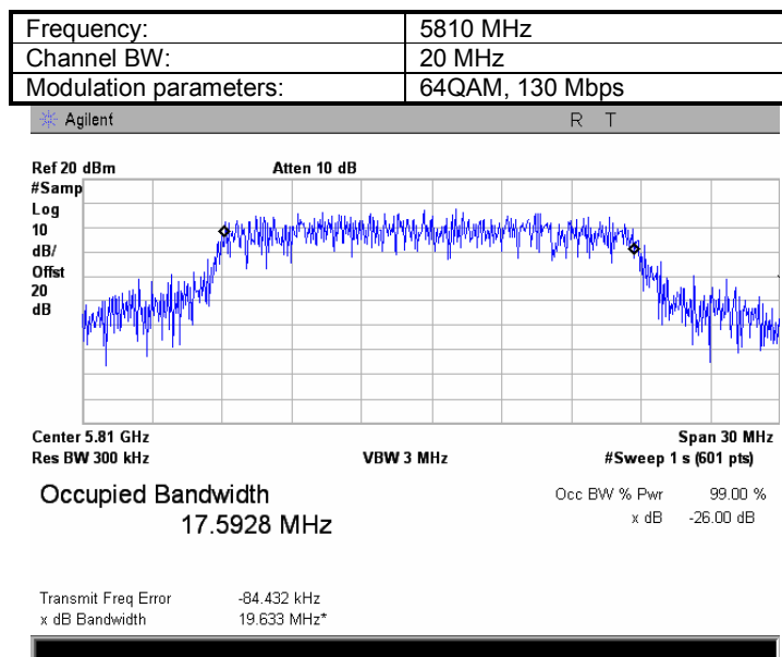
Plot 8.1.14 The 99%power bandwidth test result at low frequency
