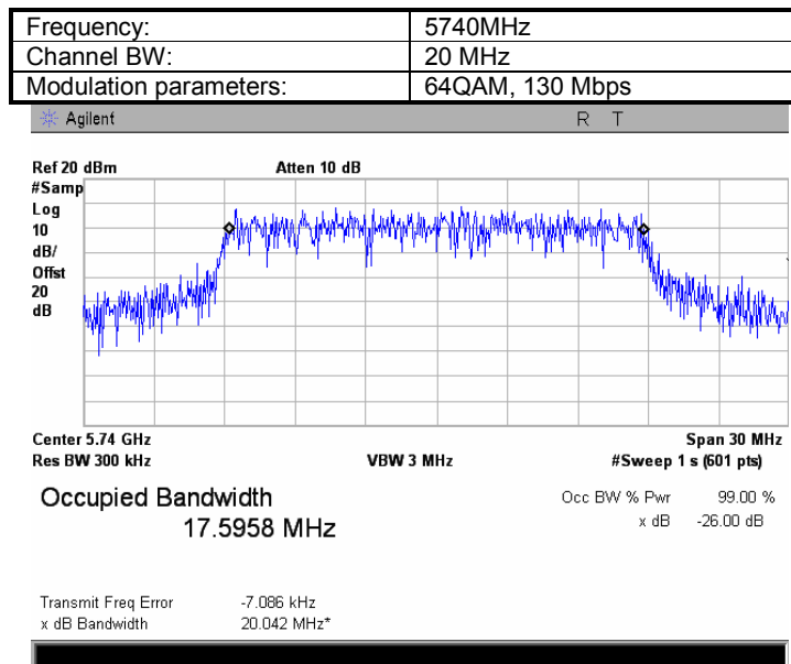
Plot 8.1.10 The 99%power bandwidth test result at low frequency
