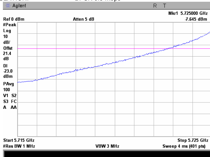
Plot 7.4.50 Conducted spurious emission measurements at the band edge
