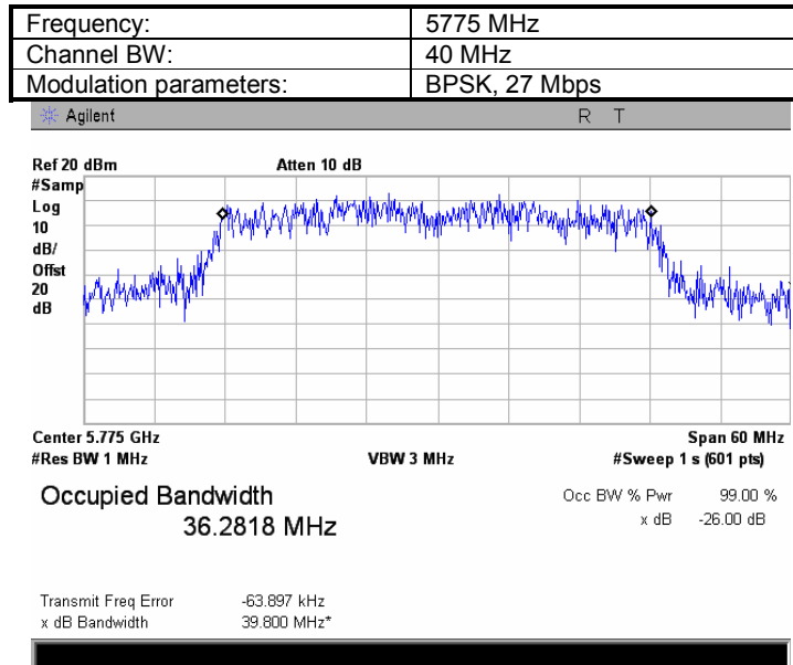
Plot 8.1.3 The 99%power bandwidth test result at low frequency
