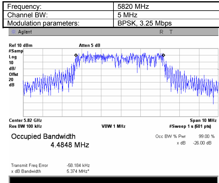
Plot 8.1.32 The 99%power bandwidth test result at low frequency
