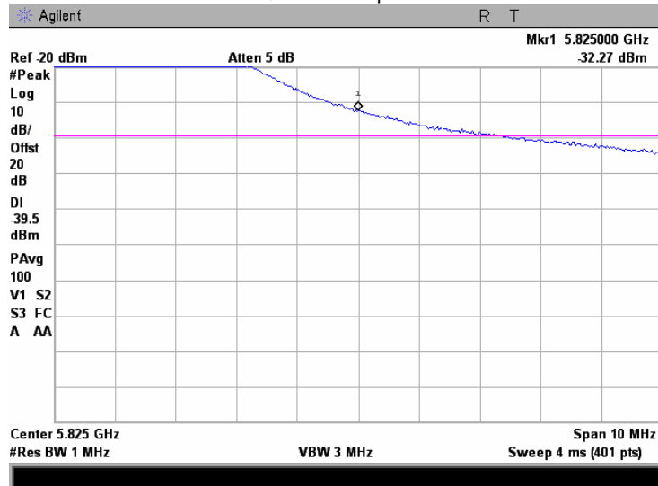
Plot 7.5.12 Conducted spurious emission measurements at the band edges
