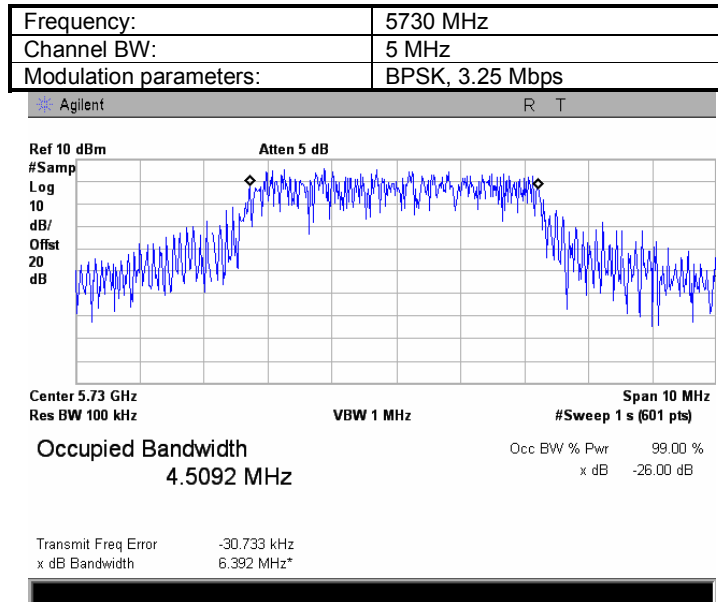
Plot 8.1.28 The 99%power bandwidth test result at low frequency
