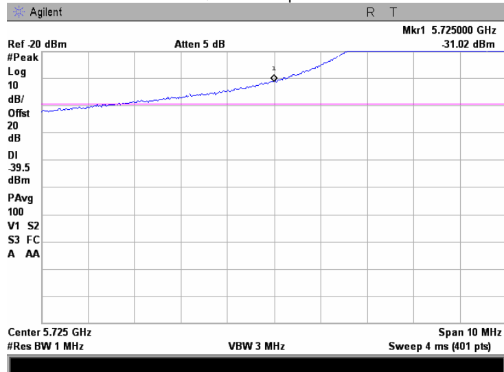
Plot 7.5.4 Conducted spurious emission measurements at the low band edge
