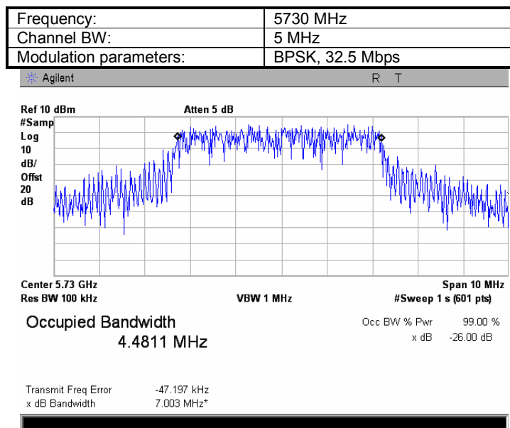
Plot 8.1.28 The 99%power bandwidth test result at low frequency
