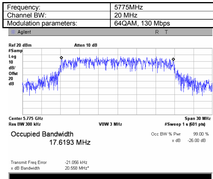
Plot 8.1.12 The 99%power bandwidth test result at low frequency
