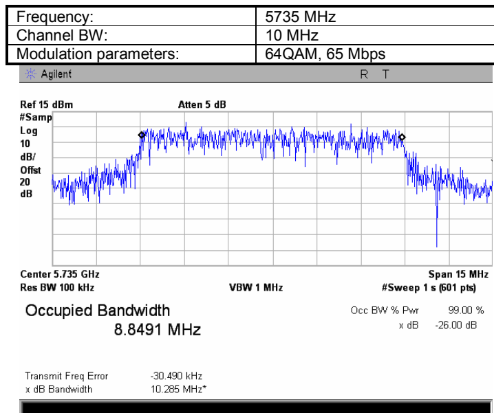
Plot 8.1.20 The 99%power bandwidth test result at low frequency
