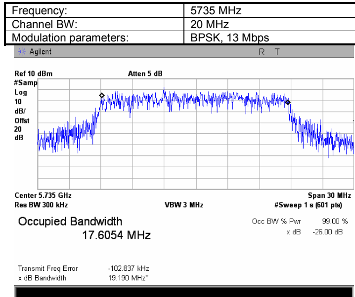
Plot 8.1.8 The 99%power bandwidth test result at low frequency
