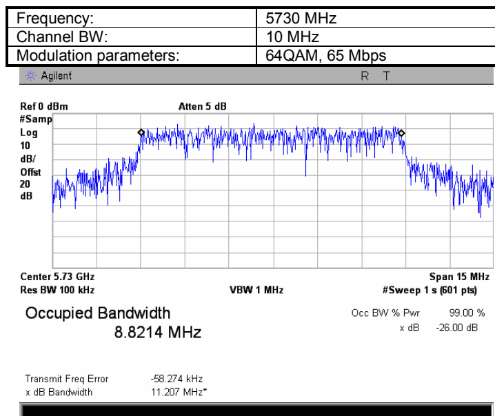
Plot 8.1.18 The 99%power bandwidth test result at low frequency
