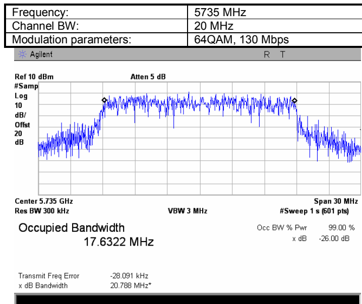
Plot 8.1.8 The 99%power bandwidth test result at low frequency
