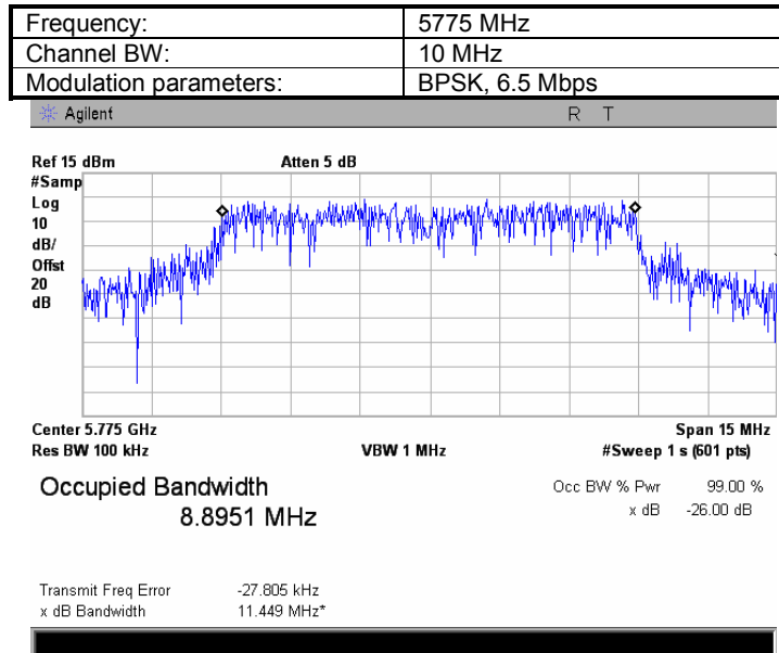
Plot 8.1.22 The 99%power bandwidth test result at low frequency
