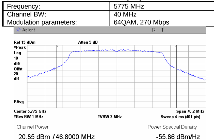
Plot 7.1.215 Peak output power
