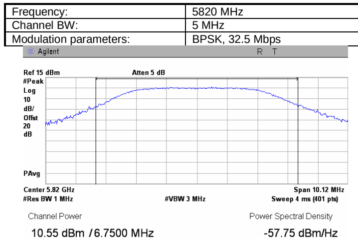
Plot 7.1.203 Peak output power
