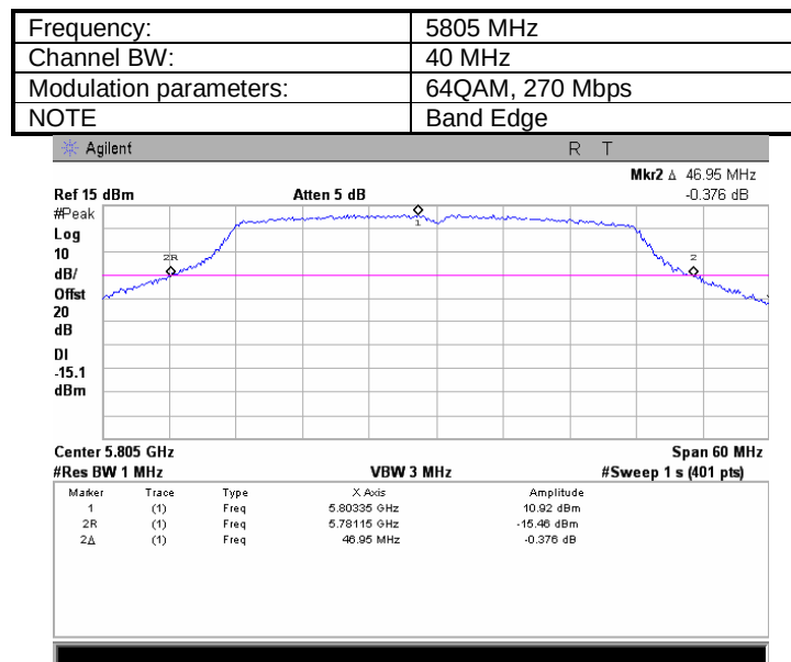
Plot 7.1.16 The 26 dB emission bandwidth
