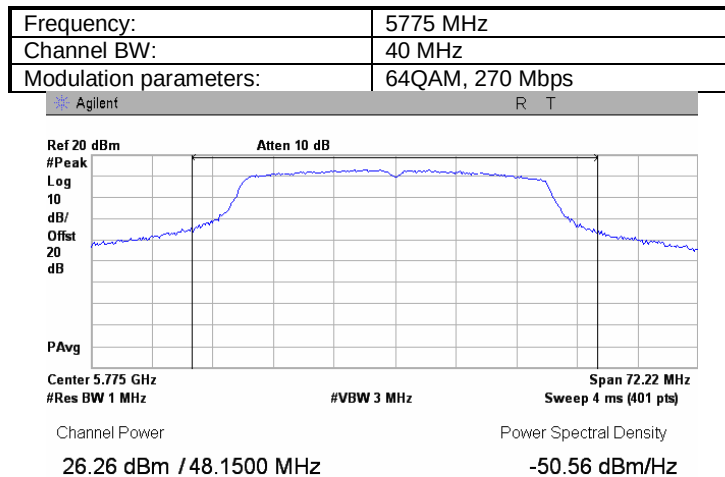
Plot 7.1.11 Peak output power
