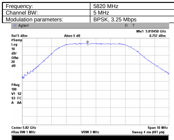
Plot 7.1.202 The 26 dB emission bandwidth
