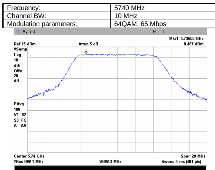
Plot 7.1.156 Peak spectral power density
