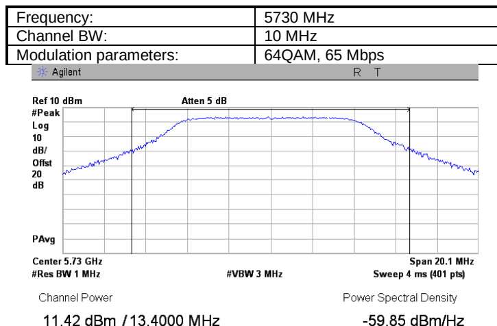
Plot 7.1.53 Peak output power
