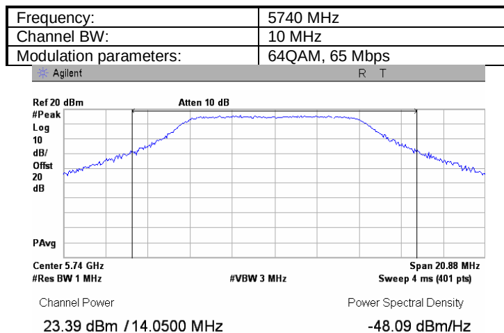
Plot 7.1.155 Peak output power
