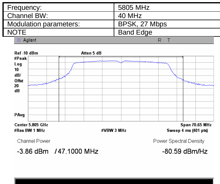
Plot 7.1.218 Peak output power
