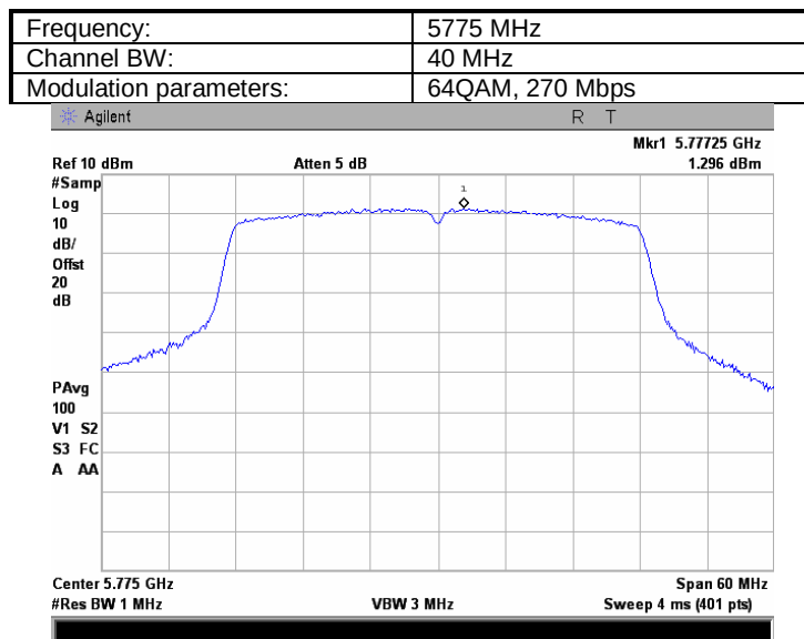
Plot 7.1.108 Peak spectral power density
