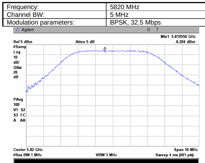
Plot 7.1.204 Peak spectral power density
