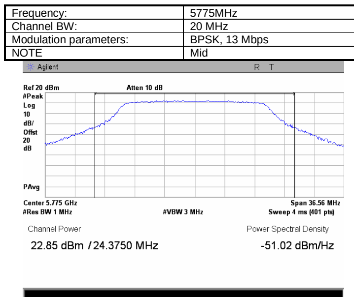
Plot 7.1.32 Peak output power
