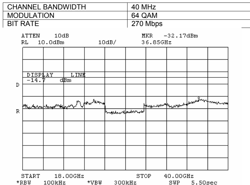
Plot 7.3.166 Spurious emission measurements in 18000 – 40000 MHz range at low carrier frequency, Antenna 2
