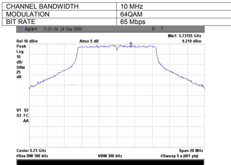
Plot 7.3.2 The highest emission level within the assigned band at low carrier frequency, combined
