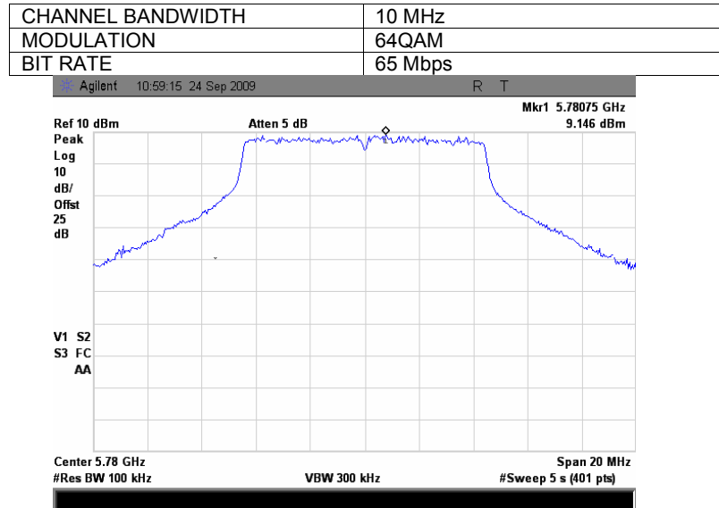
Plot 7.3.3 The highest emission level within the assigned band at mid carrier frequency, combined
