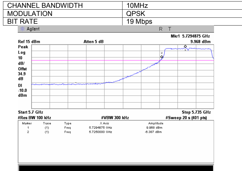
Plot 7.3.19 Spurious emission measurements in 5700 – 5725 MHz range at low carrier frequency, combined
