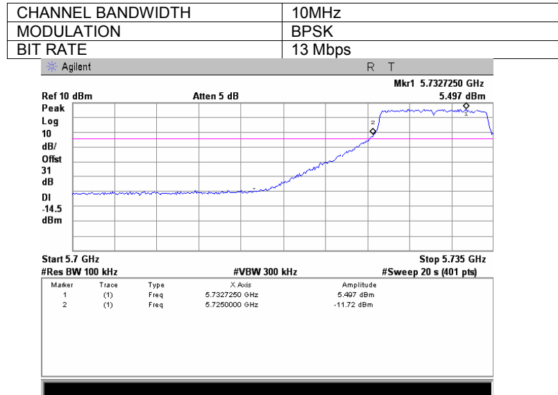
Plot 7.3.81 Spurious emission measurements in 5700 – 5725 MHz range at low carrier frequency, Antenna 1
