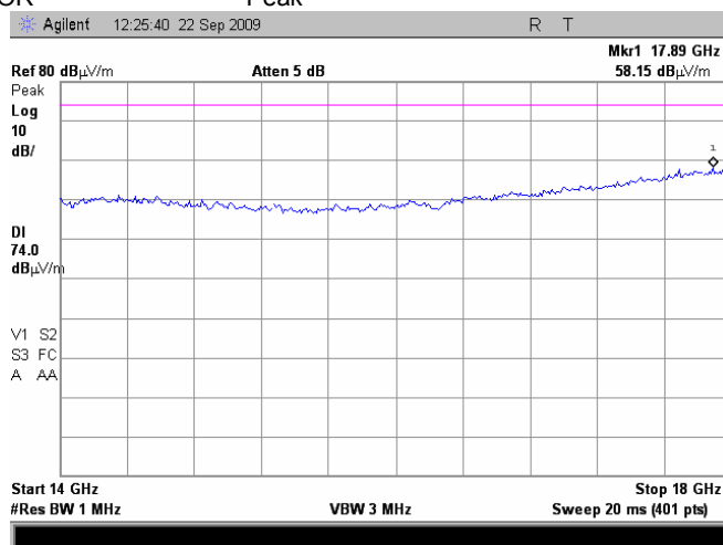
Plot 7.4.52 Radiated emission measurements from 14000 to 18000 MHz at the low carrier frequency
