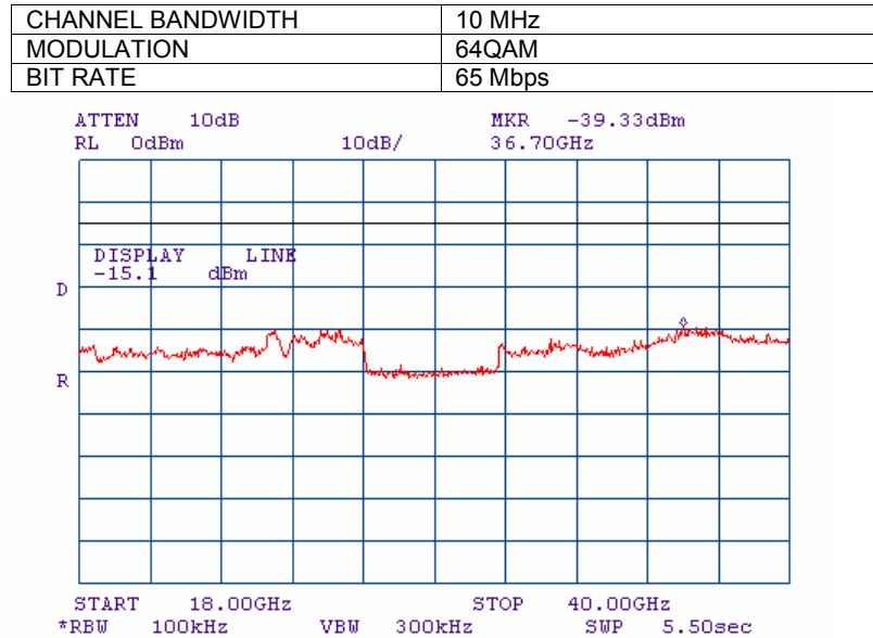
Plot 7.3.78 Spurious emission measurements in 18000 – 40000 MHz range at high carrier frequency, Antenna 2
