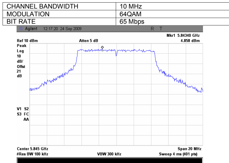
Plot 7.3.43 The highest emission level within the assigned band at high carrier frequency, Antenna 2
