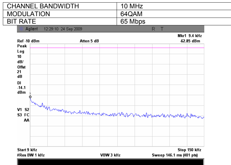
Plot 7.3.45 Spurious emission measurements in 9 - 150 kHz range at low carrier frequency, Antenna 2
