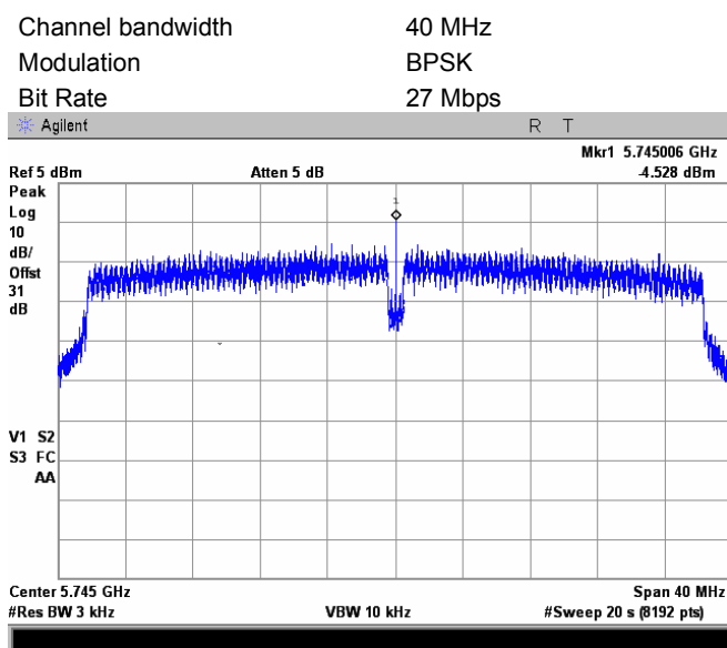
Plot 7.6.33 Peak spectral power density at low frequency zoomed at the peak, Antenna 1
