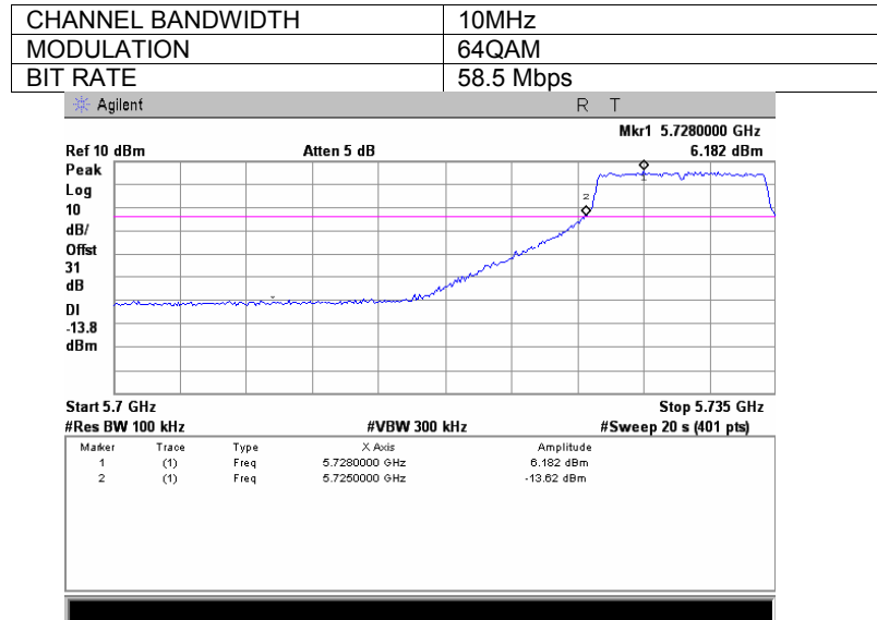
Plot 7.3.86 Spurious emission measurements in 5700 – 5725 MHz range at low carrier frequency, Antenna 1
