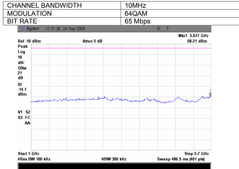
Plot 7.3.54 Spurious emission measurements in 1000 – 5700 MHz range at low carrier frequency, Antenna 2
