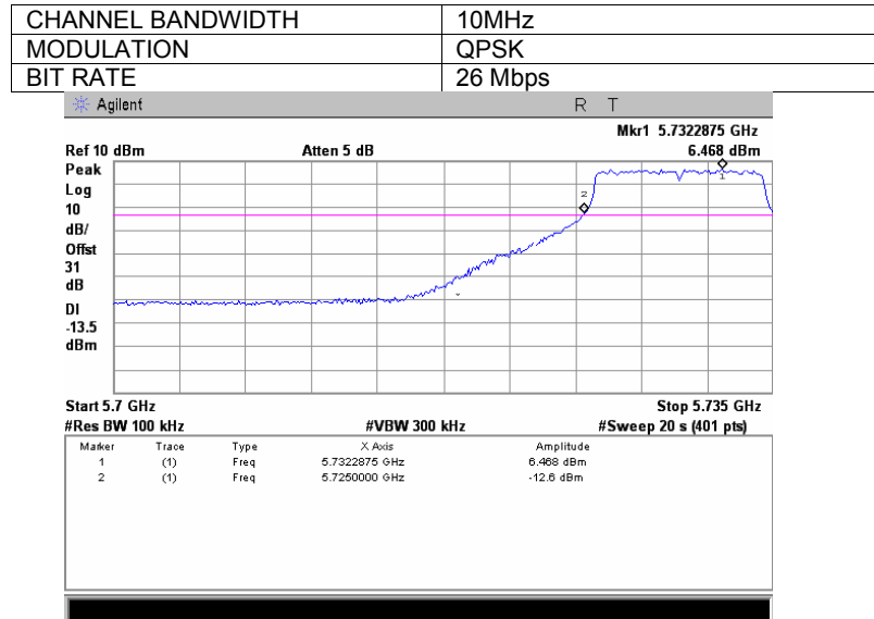
Plot 7.3.83 Spurious emission measurements in 5700 – 5725 MHz range at low carrier frequency, Antenna 1
