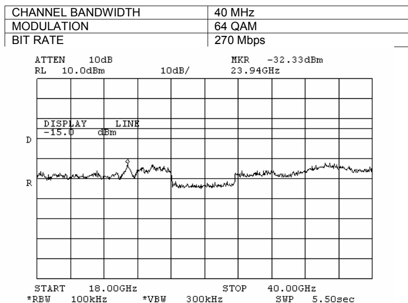
Plot 7.3.167 Spurious emission measurements in 18000 – 40000 MHz range at mid carrier frequency, Antenna 2
