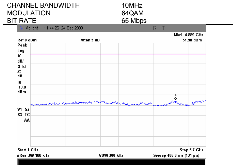
Plot 7.3.15 Spurious emission measurements in 1000 – 5700 MHz range at low carrier frequency, combined
