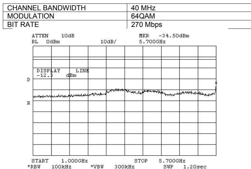
Plot 7.3.107 Spurious emission measurements in 1000 – 5700 MHz range at low carrier frequency, combined
