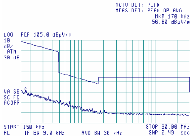
Plot 7.4.18 Radiated emission measurements from 0.15 to 30 MHz at the high carrier frequency
