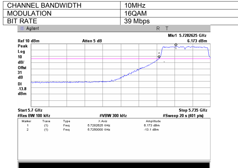
Plot 7.3.84 Spurious emission measurements in 5700 – 5725 MHz range at low carrier frequency, Antenna 1
