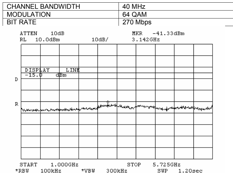
Plot 7.3.153 Spurious emission measurements in 1000 – 5725 MHz range at mid carrier frequency, Antenna 2
