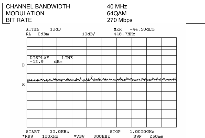
Plot 7.3.106 Spurious emission measurements in 30 - 1000 MHz range at high carrier frequency, combined
