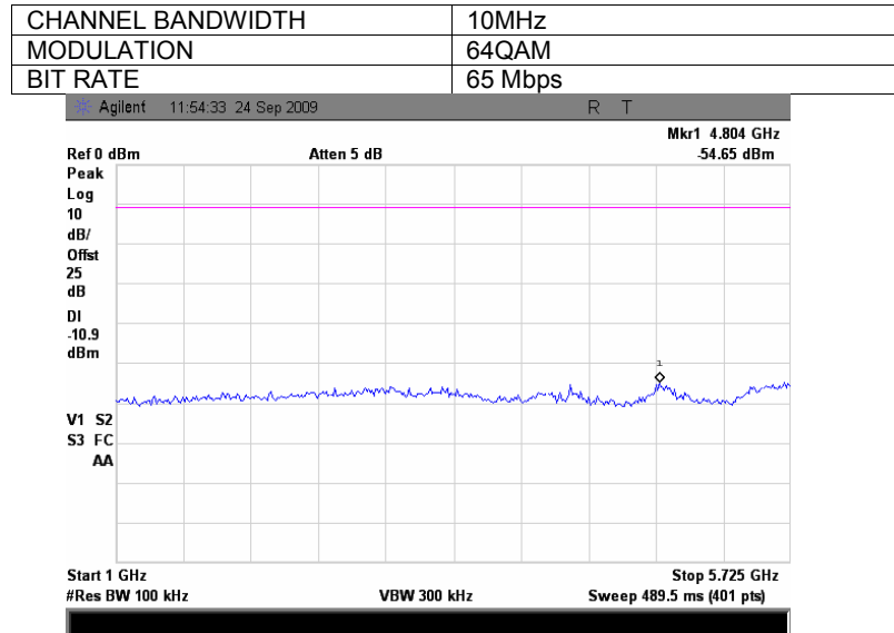
Plot 7.3.24 Spurious emission measurements in 1000 – 5725 MHz range at mid carrier frequency, combined
