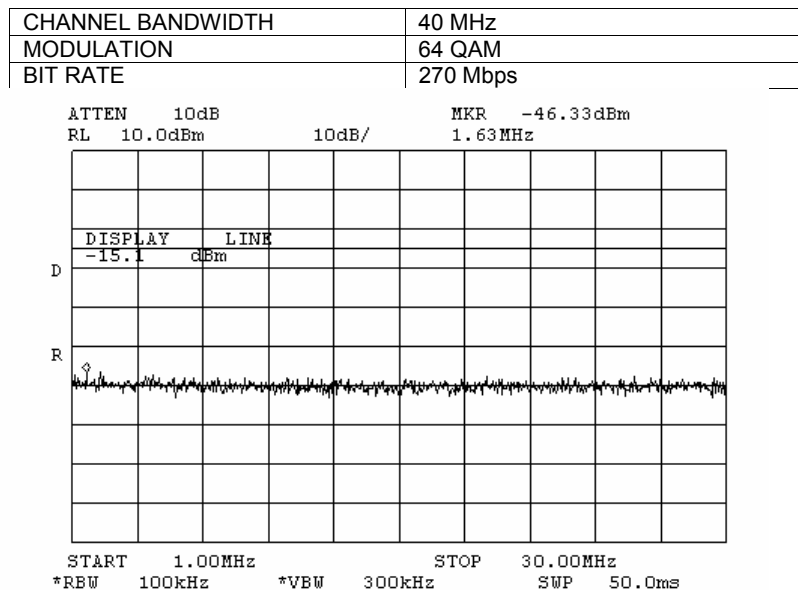
Plot 7.3.140 Spurious emission measurements in 1 - 30 MHz range at high carrier frequency, Antenna 2
