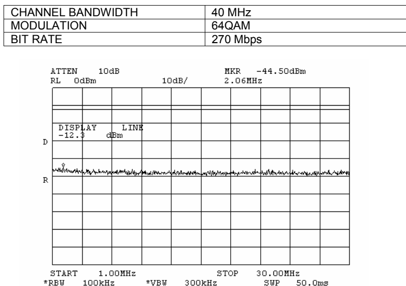
Plot 7.3.101 Spurious emission measurements in 1 - 30 MHz range at low carrier frequency, combined
