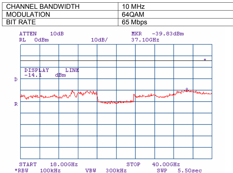
Plot 7.3.76 Spurious emission measurements in 18000 – 40000 MHz range at low carrier frequency, Antenna 2
