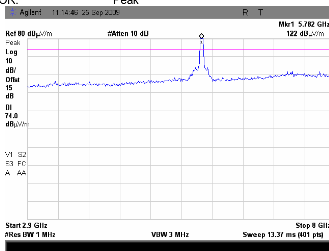
Plot 7.5.16 Radiated emission measurements from 2900 to 8000 MHz at the mid carrier frequency
