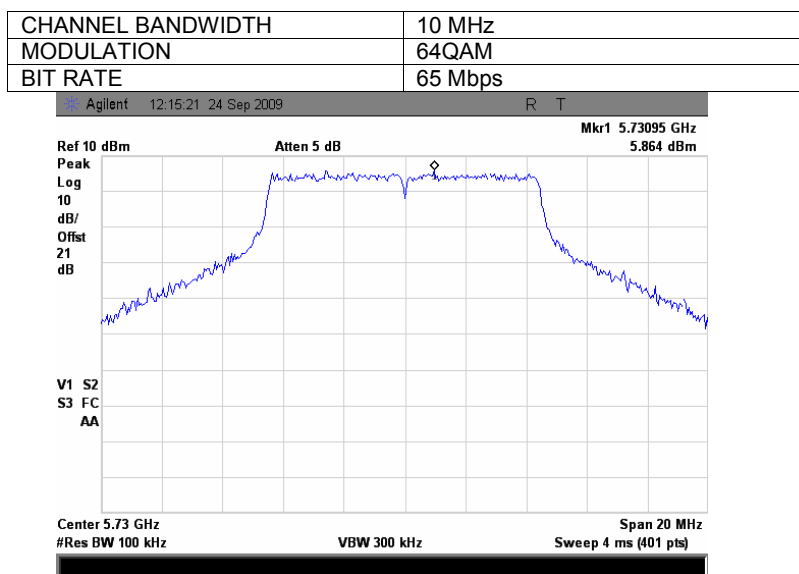
Plot 7.3.40 The highest emission level within the assigned band at low carrier frequency, Antenna 2
