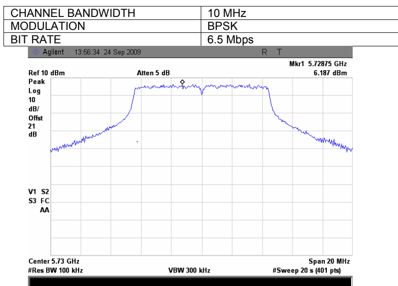
Plot 7.3.41 The highest emission level within the assigned band at low carrier frequency, Antenna 2
