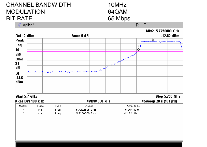
Plot 7.3.79 Spurious emission measurements in 5700 – 5725 MHz range at low carrier frequency, Antenna 1
