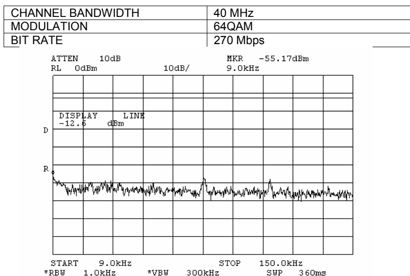
Plot 7.3.96 Spurious emission measurements in 9 - 150 kHz range at mid carrier frequency, combined
