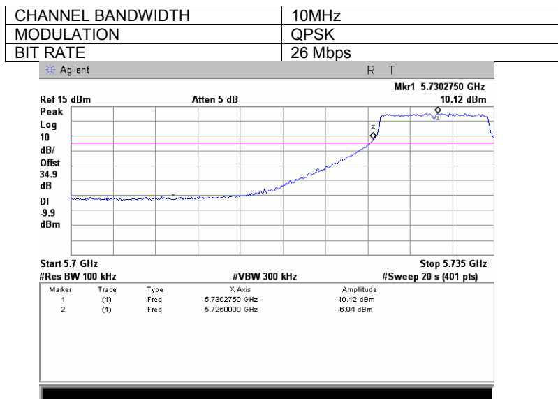
Plot 7.3.20 Spurious emission measurements in 5700 – 5725 MHz range at low carrier frequency, combined
