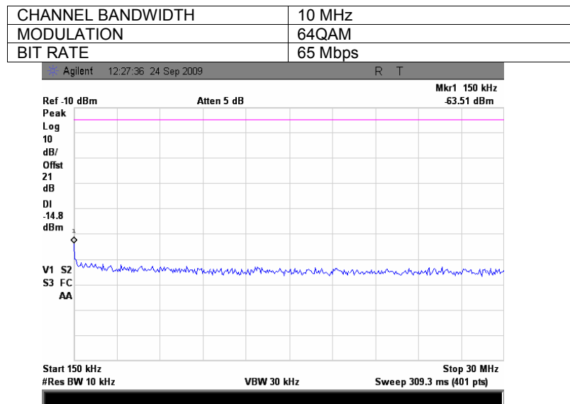
Plot 7.3.49 Spurious emission measurements in 0.15 - 30 MHz range at mid carrier frequency, Antenna 2
