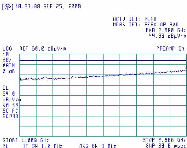
Plot 7.5.12 Radiated emission measurements from 1000 to 2900 MHz at the high carrier frequency
