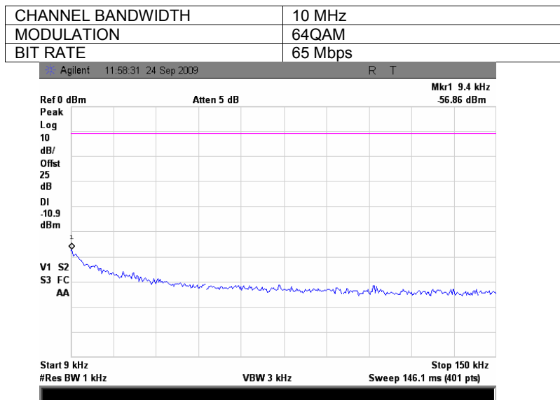
Plot 7.3.8 Spurious emission measurements in 9 - 150 kHz range at high carrier frequency, combined
