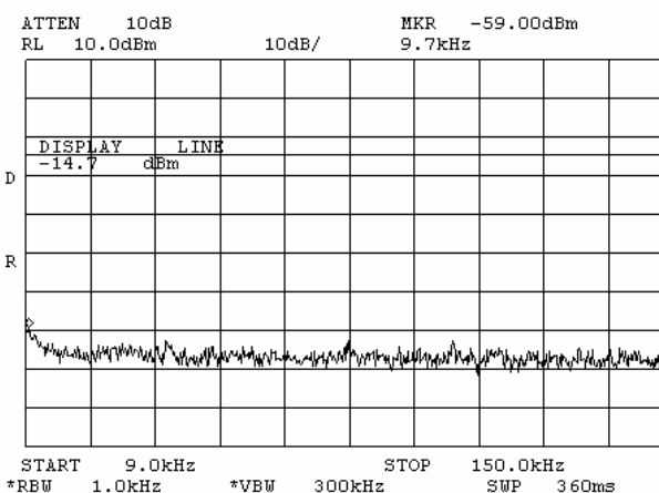
Plot 7.3.133 Spurious emission measurements in 9 - 150 kHz range at mid carrier frequency, Antenna 2
