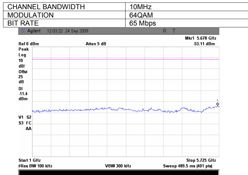
Plot 7.3.25 Spurious emission measurements in 1000 – 5725 MHz range at high carrier frequency, combined Tx chains testing
