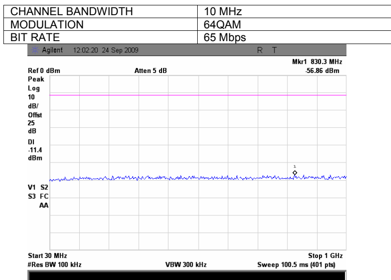
Plot 7.3.14 Spurious emission measurements in 30 - 1000 MHz range at high carrier frequency, combined
