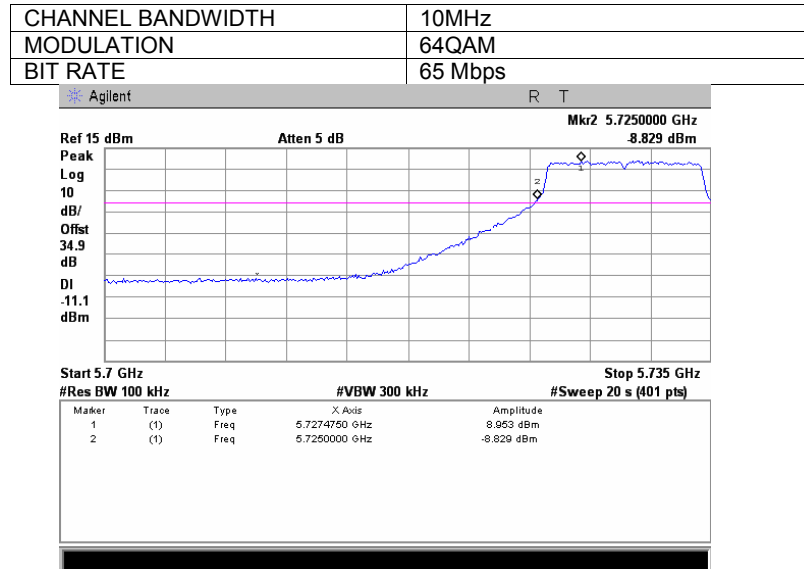
Plot 7.3.16 Spurious emission measurements in 5700 – 5725 MHz range at low carrier frequency, combined
