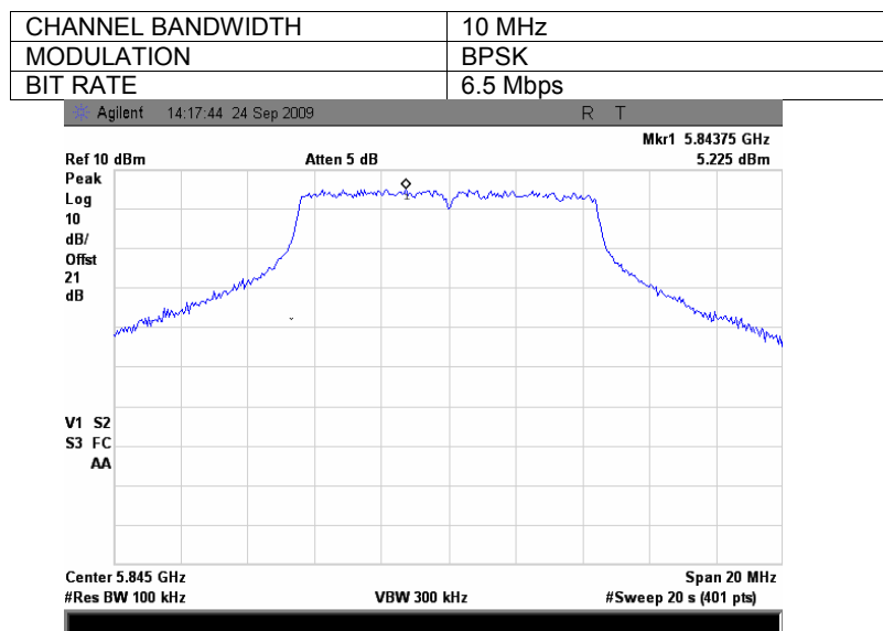
Plot 7.3.44 The highest emission level within the assigned band at high carrier frequency, Antenna 2
