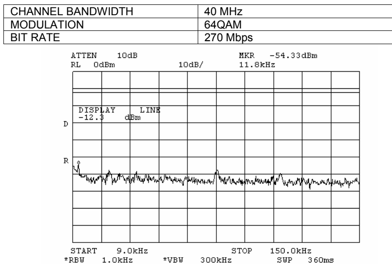
Plot 7.3.95 Spurious emission measurements in 9 - 150 kHz range at low carrier frequency, combined
