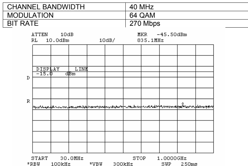
Plot 7.3.142 Spurious emission measurements in 30 - 1000 MHz range at mid carrier frequency, Antenna 2
