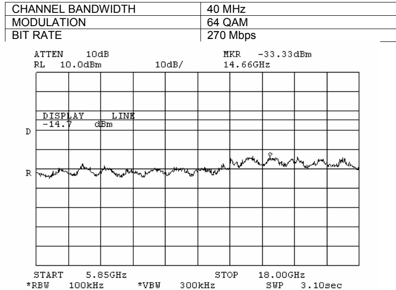
Plot 7.3.155 Spurious emission measurements in 5850 – 18000 MHz range at low carrier frequency, Antenna 2
