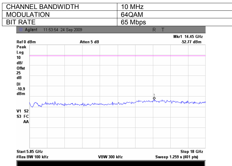
Plot 7.3.27 Spurious emission measurements in 5850 – 18000 MHz range at mid carrier frequency, combined
