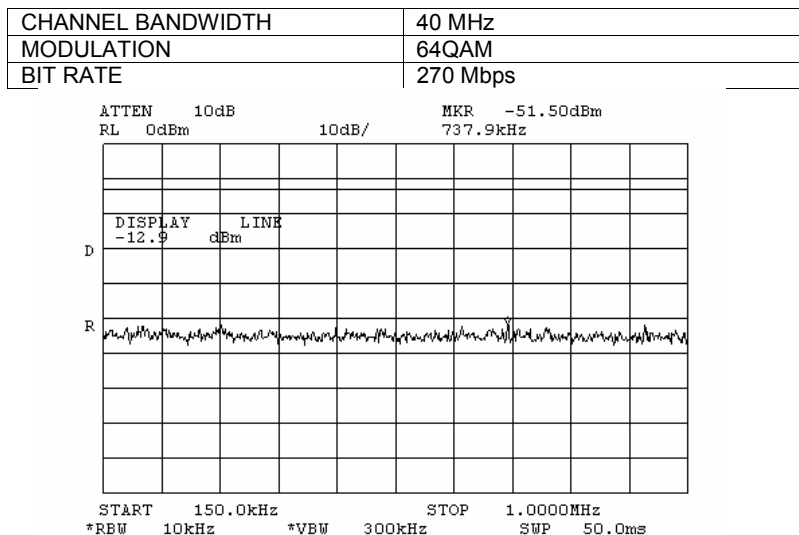
Plot 7.3.100 Spurious emission measurements in 0.15 - 1 MHz range at high carrier frequency, combined
