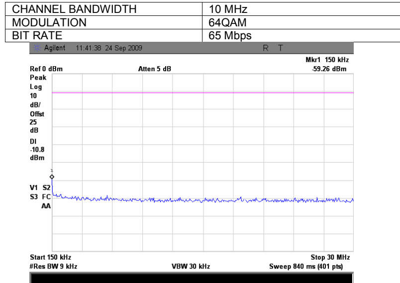
Plot 7.3.10 Spurious emission measurements in 0.15 - 30 MHz range at mid carrier frequency, combined
