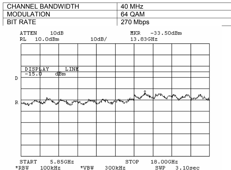
Plot 7.3.156 Spurious emission measurements in 5850 – 18000 MHz range at mid carrier frequency, Antenna 2
