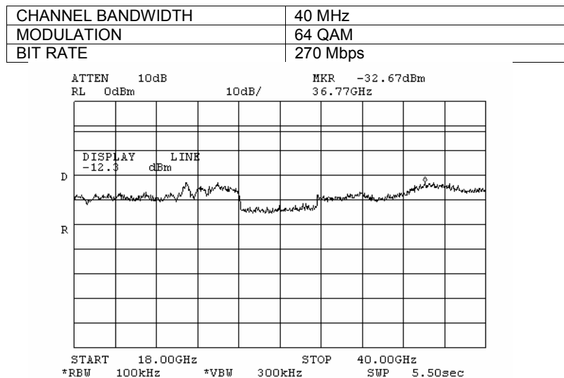
Plot 7.3.129 Spurious emission measurements in 18000 – 40000 MHz range at low carrier frequency, combined
