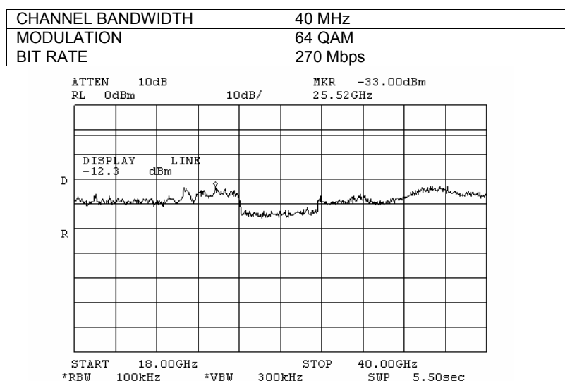
Plot 7.3.130 Spurious emission measurements in 18000 – 40000 MHz range at mid carrier frequency, combined
