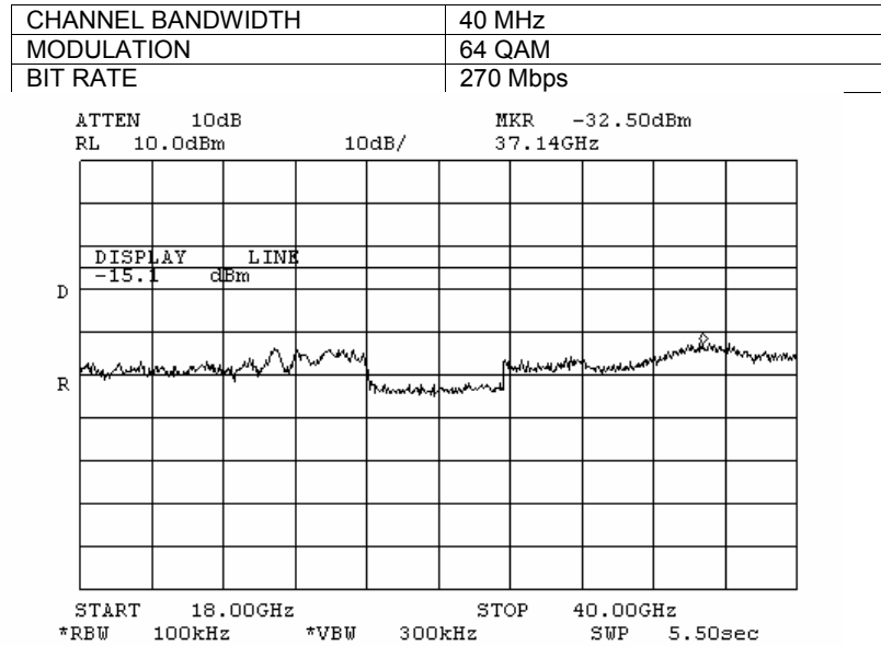
Plot 7.3.168 Spurious emission measurements in 18000 – 40000 MHz range at high carrier frequency, Antenna 2
