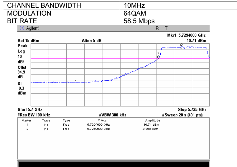
Plot 7.3.23 Spurious emission measurements in 5700 – 5725 MHz range at low carrier frequency, combined
