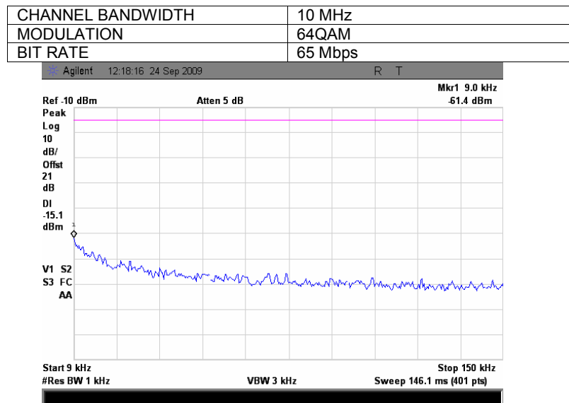
Plot 7.3.47 Spurious emission measurements in 9 - 150 kHz range at high carrier frequency, Antenna 2
