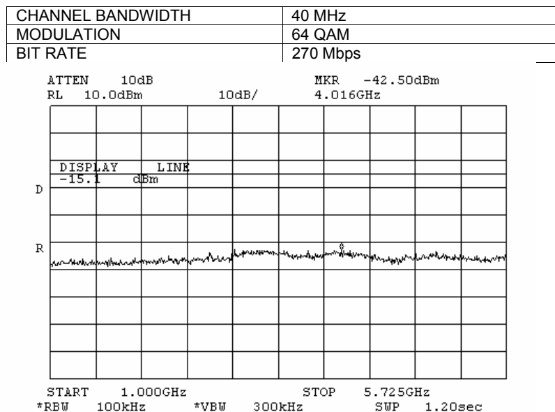
Plot 7.3.154 Spurious emission measurements in 1000 – 5725 MHz range at high carrier frequency, Antenna 2
