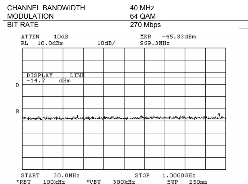
Plot 7.3.141 Spurious emission measurements in 30 - 1000 MHz range at low carrier frequency, Antenna 2
