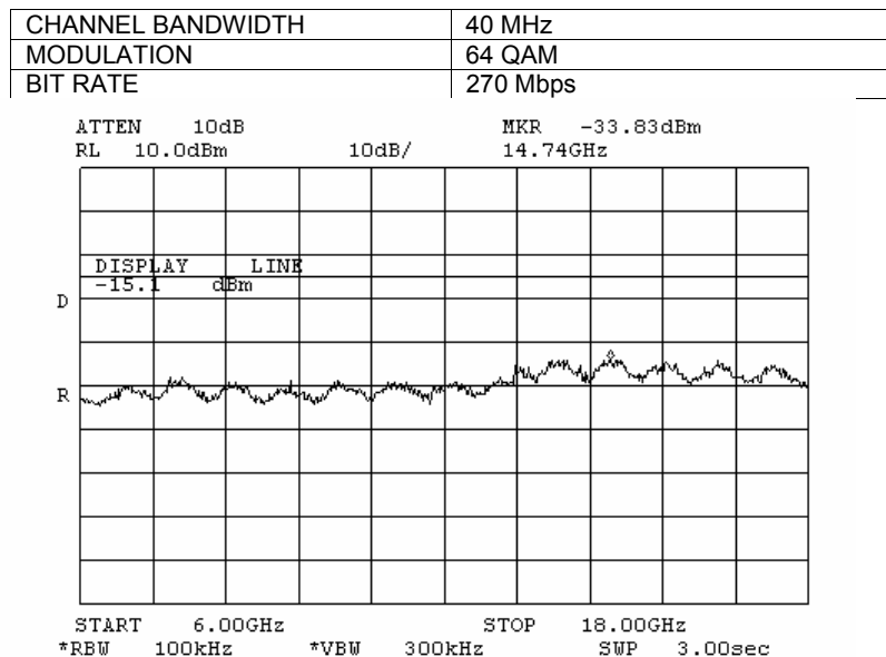
Plot 7.3.165 Spurious emission measurements in 6000 – 18000 MHz range at high carrier frequency, Antenna 2
