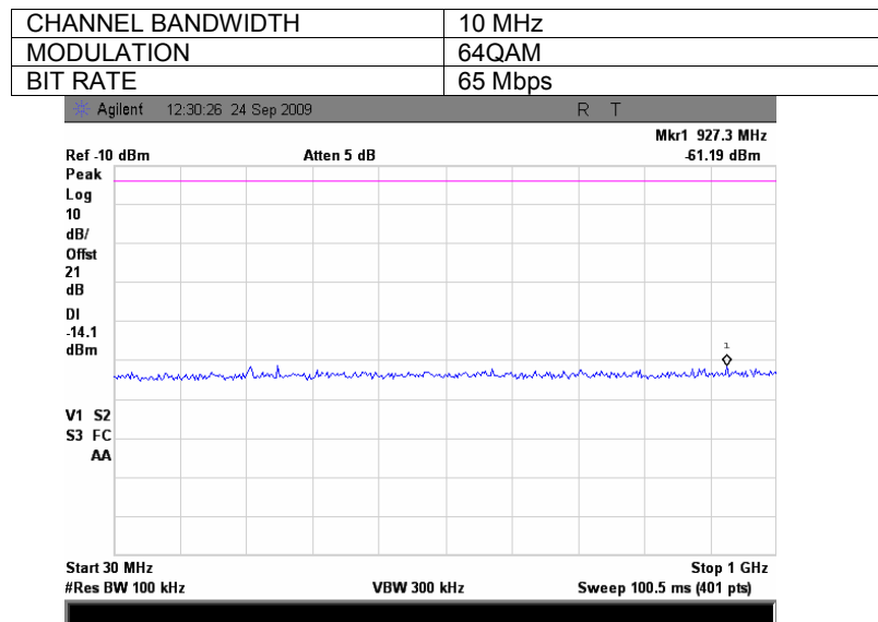
Plot 7.3.51 Spurious emission measurements in 30 - 1000 MHz range at low carrier frequency, Antenna 2
