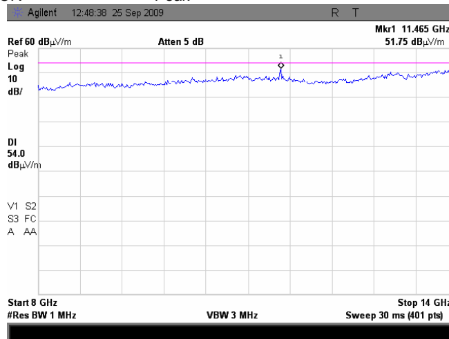
Plot 7.5.20 Radiated emission measurements from 8000 to 14000 MHz at the low carrier frequency
