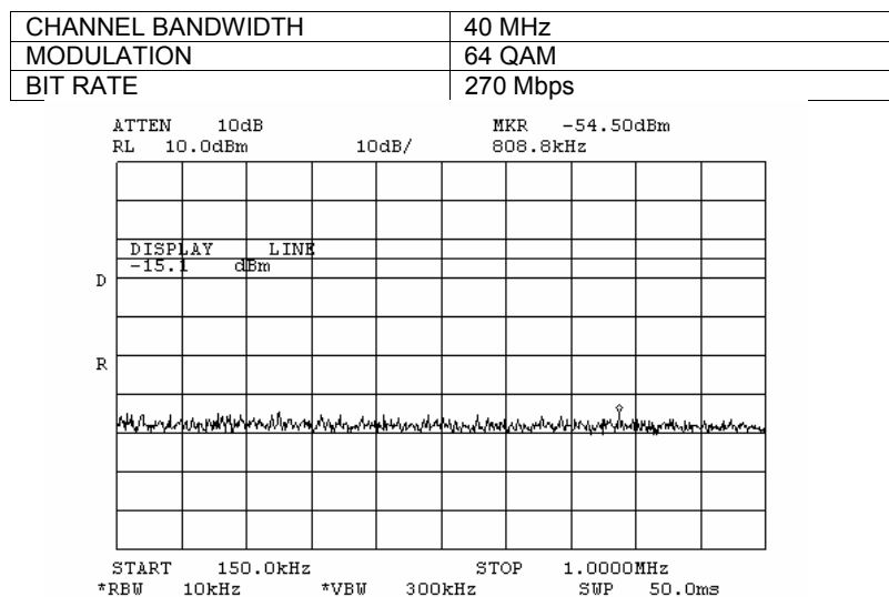
Plot 7.3.137 Spurious emission measurements in 0.15 - 1 MHz range at high carrier frequency, Antenna 2
