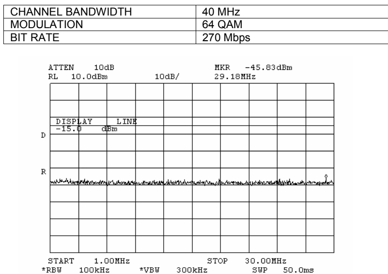
Plot 7.3.139 Spurious emission measurements in 1 - 30 MHz range at mid carrier frequency, Antenna 2
