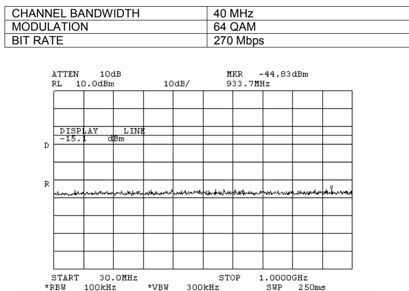
Plot 7.3.143 Spurious emission measurements in 30 - 1000 MHz range at high carrier frequency, Antenna 2
