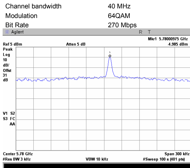
Plot 7.6.41 Peak spectral power density at mid frequency zoomed at the peak, Antenna 1
