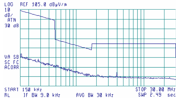
Plot 7.5.6 Radiated emission measurements from 0.15 to 30 MHz at the high carrier frequency
