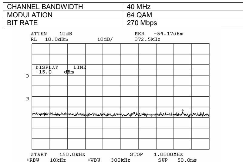
Plot 7.3.136 Spurious emission measurements in 0.15 - 1 MHz range at mid carrier frequency, Antenna 2
