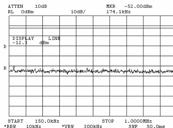
Plot 7.3.99 Spurious emission measurements in 0.15 - 1 MHz range at mid carrier frequency, combined
