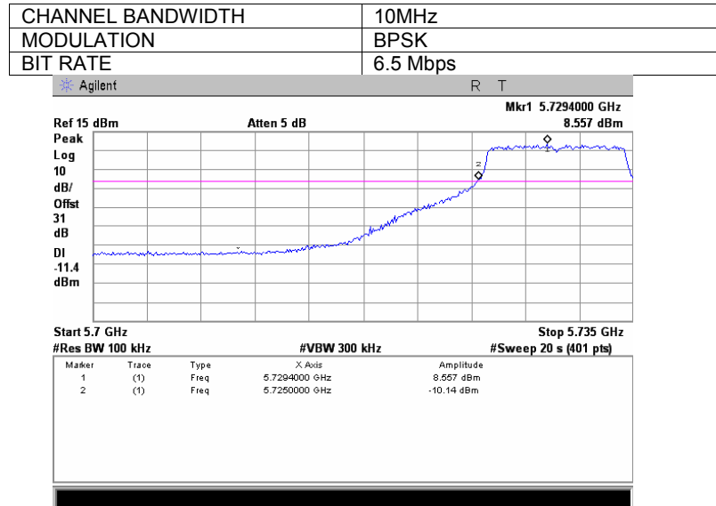
Plot 7.3.56 Spurious emission measurements in 5700 – 5725 MHz range at low carrier frequency, Antenna 2
