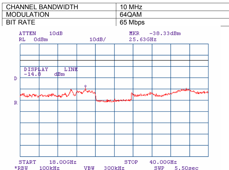
Plot 7.3.77 Spurious emission measurements in 18000 – 40000 MHz range at mid carrier frequency, Antenna 2
