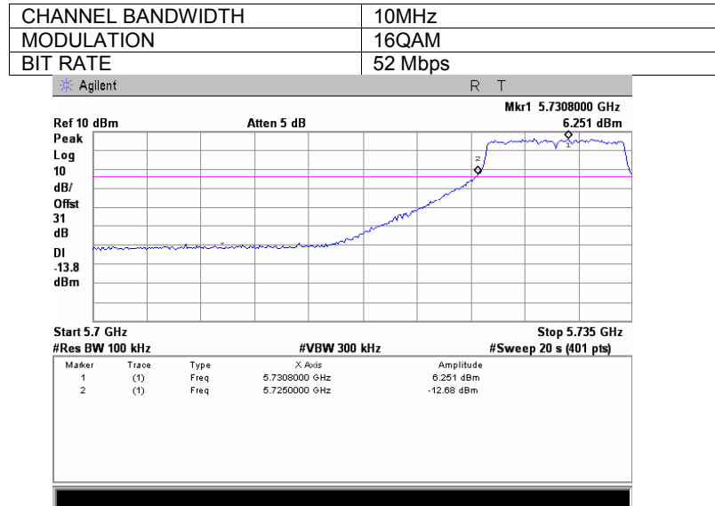
Plot 7.3.85 Spurious emission measurements in 5700 – 5725 MHz range at low carrier frequency, Antenna 1
