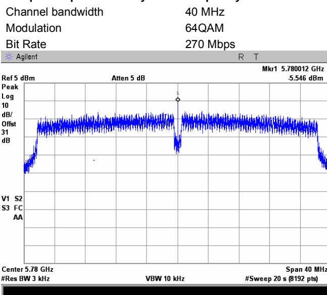
Plot 7.6.40 Peak spectral power density at mid frequency within 6 dB band, Antenna 1
