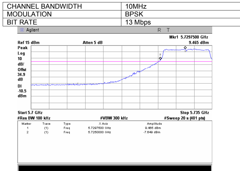
Plot 7.3.18 Spurious emission measurements in 5700 – 5725 MHz range at low carrier frequency, combined
