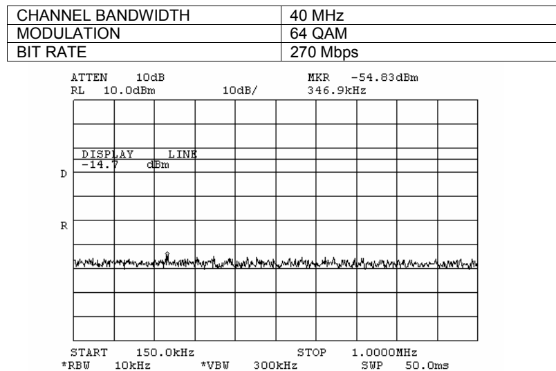
Plot 7.3.135 Spurious emission measurements in 0.15 - 1 MHz range at low carrier frequency, Antenna 2
