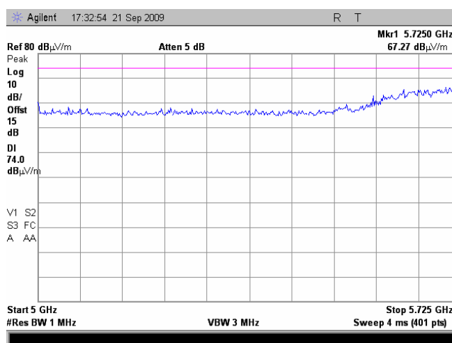
Plot 7.4.35 Radiated emission measurements from 5000 to 5725 MHz at the high carrier frequency
