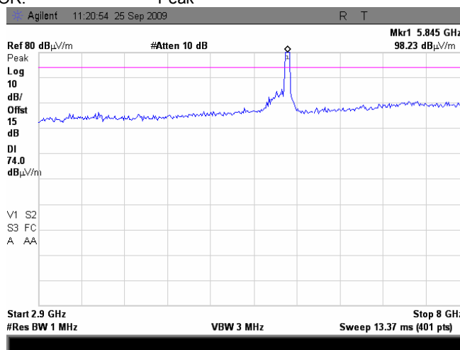
Plot 7.5.18 Radiated emission measurements from 2900 to 8000 MHz at the high carrier frequency
