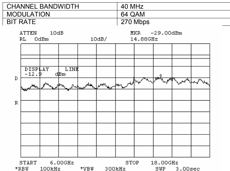
Plot 7.3.128 Spurious emission measurements in 6000 – 18000 MHz range at high carrier frequency, combined
