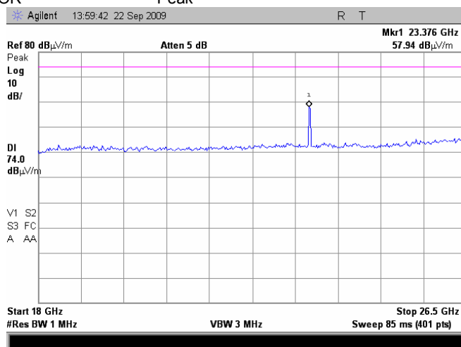
Plot 7.4.62 Radiated emission measurements from 18000 to 26500 MHz at the high carrier frequency
