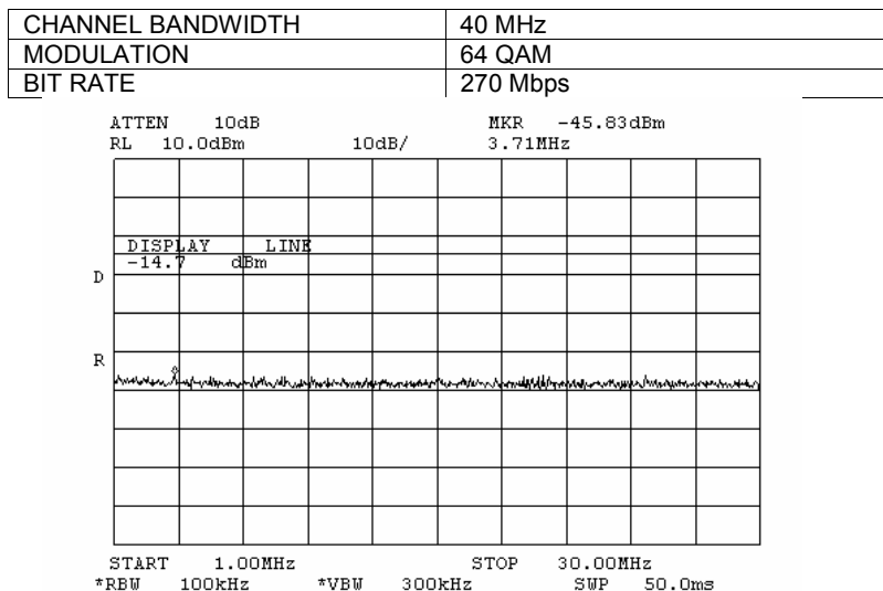
Plot 7.3.138 Spurious emission measurements in 1 - 30 MHz range at low carrier frequency, Antenna 2
