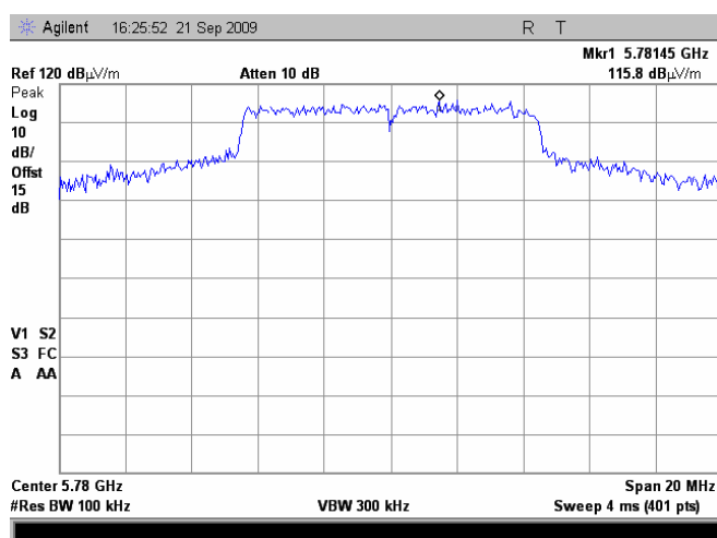
Plot 7.4.6 Radiated emission measurements at the mid carrier frequency
