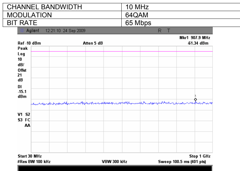
Plot 7.3.53 Spurious emission measurements in 30 - 1000 MHz range at high carrier frequency, Antenna 2
