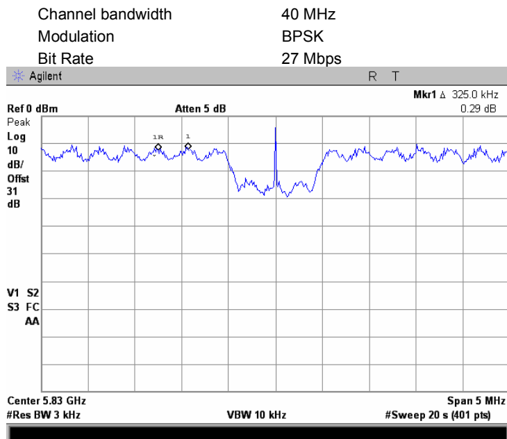
Plot 7.6.31 Peak spectral power density at low frequency zoomed, Antenna 1
