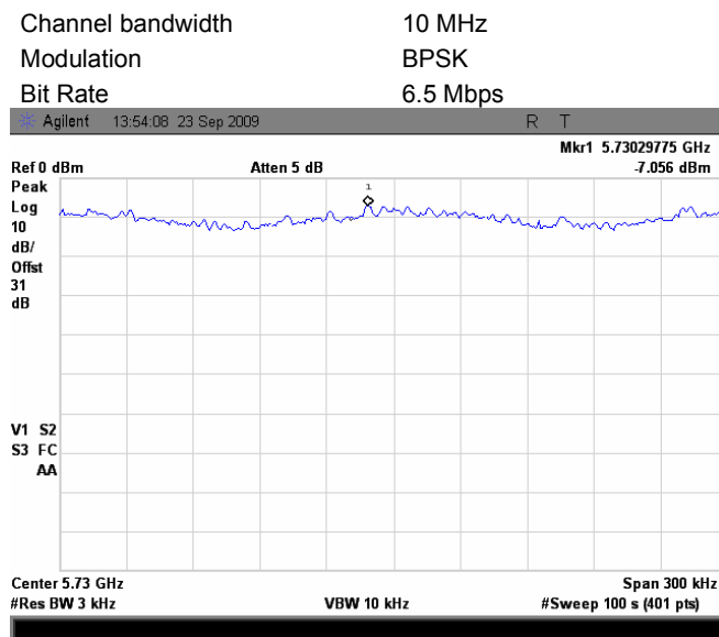
Plot 7.6.2 Peak spectral power density at low frequency zoomed at the peak, Antenna 1
