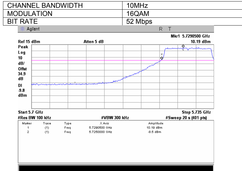
Plot 7.3.22 Spurious emission measurements in 5700 – 5725 MHz range at low carrier frequency, combined
