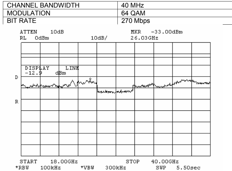
Plot 7.3.131 Spurious emission measurements in 18000 – 40000 MHz range at high carrier frequency, combined
