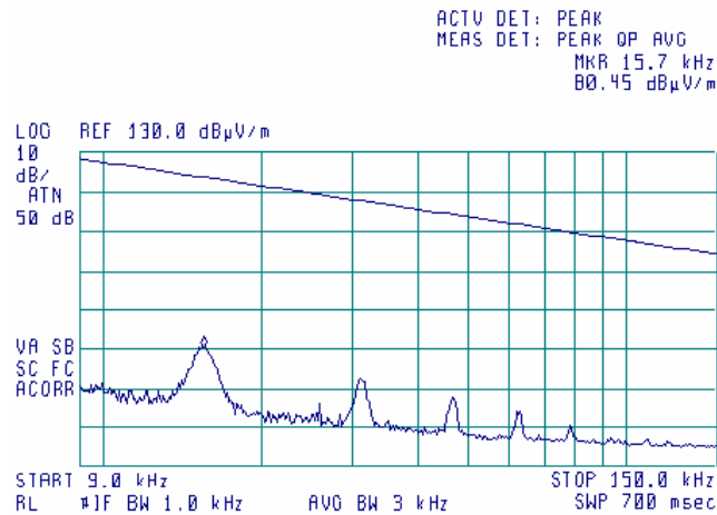
Plot 7.4.14 Radiated emission measurements from 9 to 150 kHz at the mid carrier frequency
