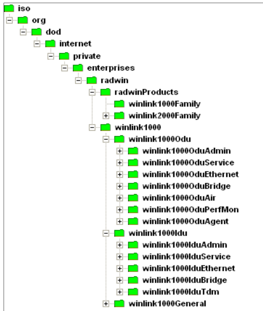
Figure F-1: Top Level Sections of the private MIB
