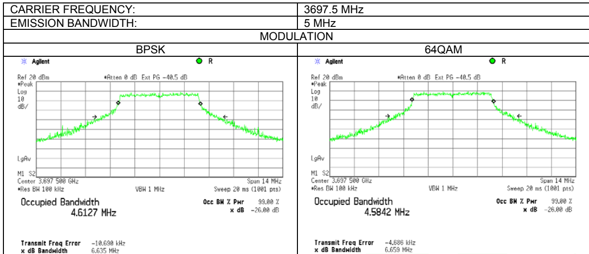
Plot 7.3.3 The 99% occupied bandwidth test results at high frequency
