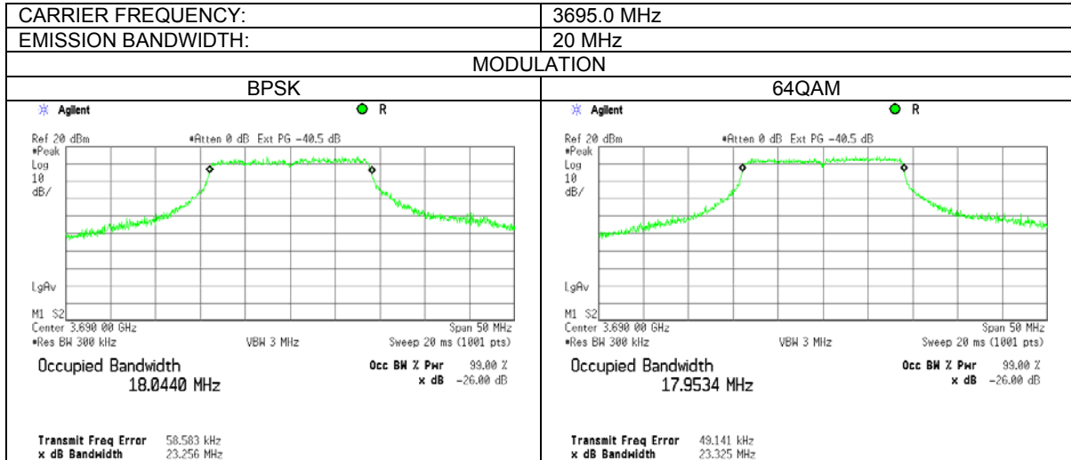
Plot 7.3.9 The 99% occupied bandwidth test results at high frequency
