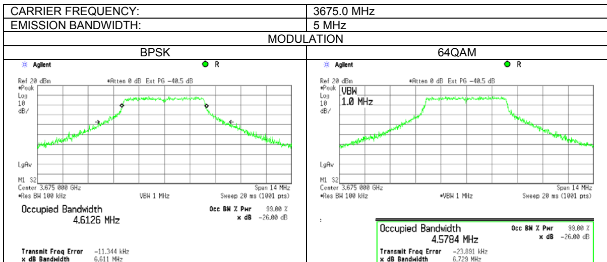
Plot 7.3.2 The 99% occupied bandwidth test results at mid frequency
