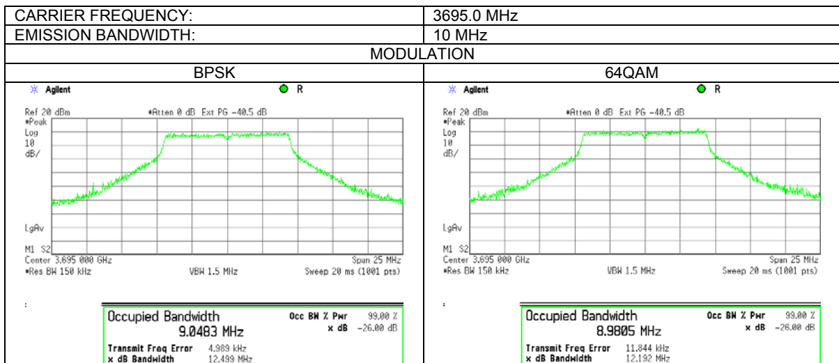
Plot 7.3.6 The 99% occupied bandwidth test results at high frequency
