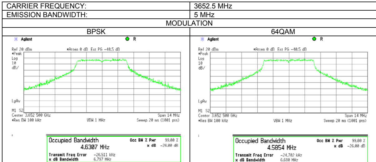
Plot 7.3.1 The 99% occupied bandwidth test results at low frequency
