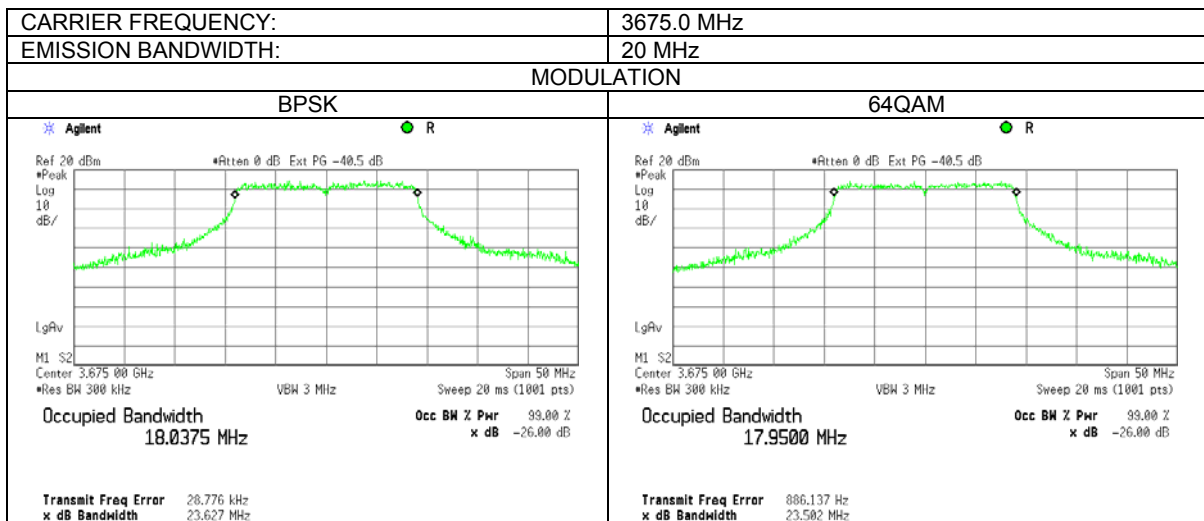
Plot 7.3.8 The 99% occupied bandwidth test results at mid frequency
