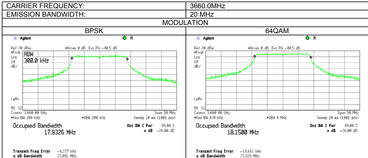
Plot 7.3.7 The 99% occupied bandwidth test results at low frequency
