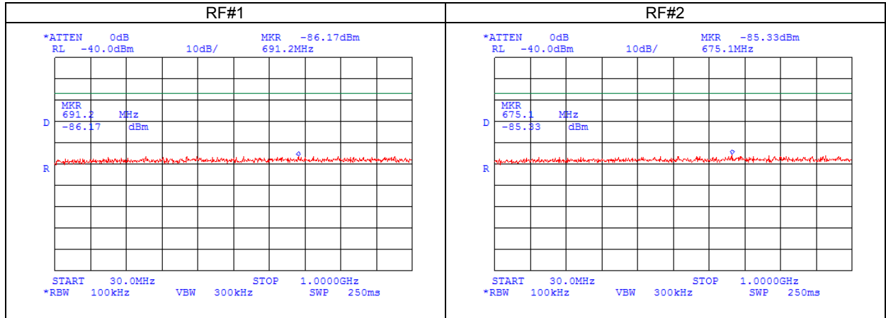
Plot 7.12.1 Spurious emission test results
