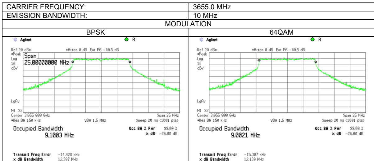
Plot 7.3.4 The 99% occupied bandwidth test results at low frequency
