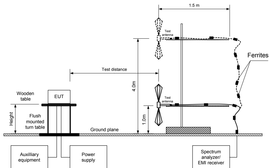
Figure 7.10.2 Setup for spurious emission field strength measurements above 30 MHz
