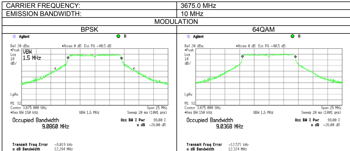
Plot 7.3.5 The 99% occupied bandwidth test results at mid frequency
