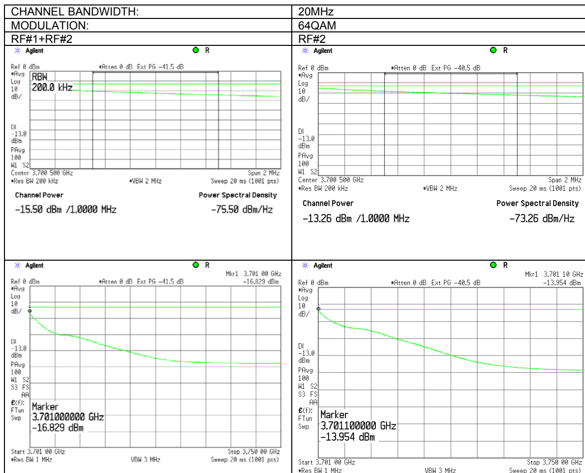
Plot 7.7.12 Spurious emission near high band edge at high carrier frequency
