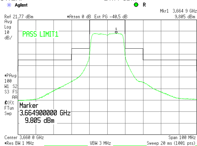
Plot 7.4.8 Emission mask test results at mid carrier frequency
