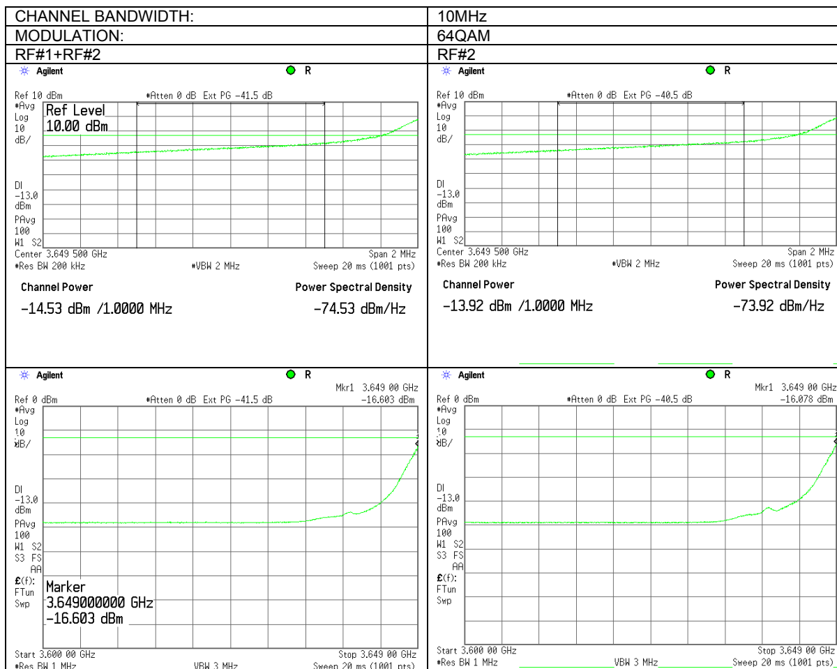
Plot 7.7.6 Spurious emission near low band edge at low carrier frequency
