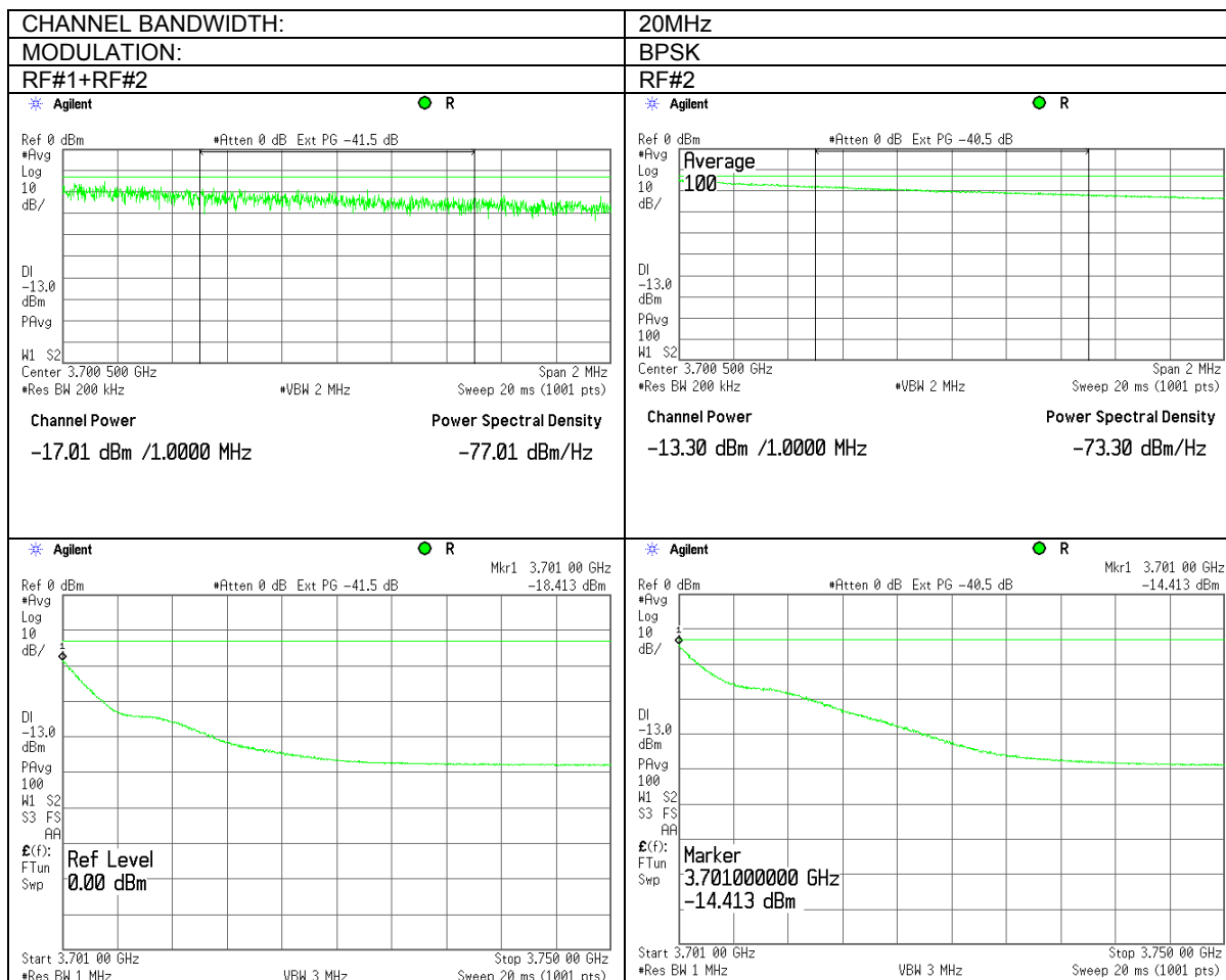
Plot 7.7.11 Spurious emission near high band edge at high carrier frequency
