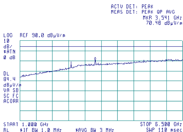
Plot 7.11.12 Radiated emission measurements in 1000 – 6500 MHz range
