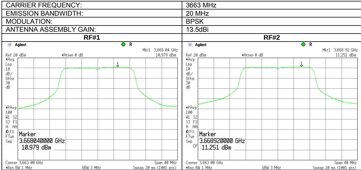
Plot 7.2.70 Peak power density test results at mid frequency
