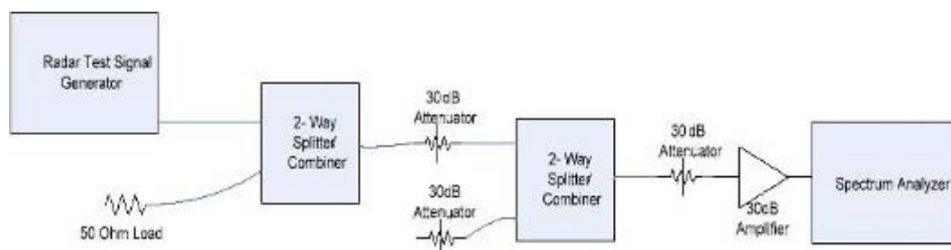
Conducted Calibration Setup
