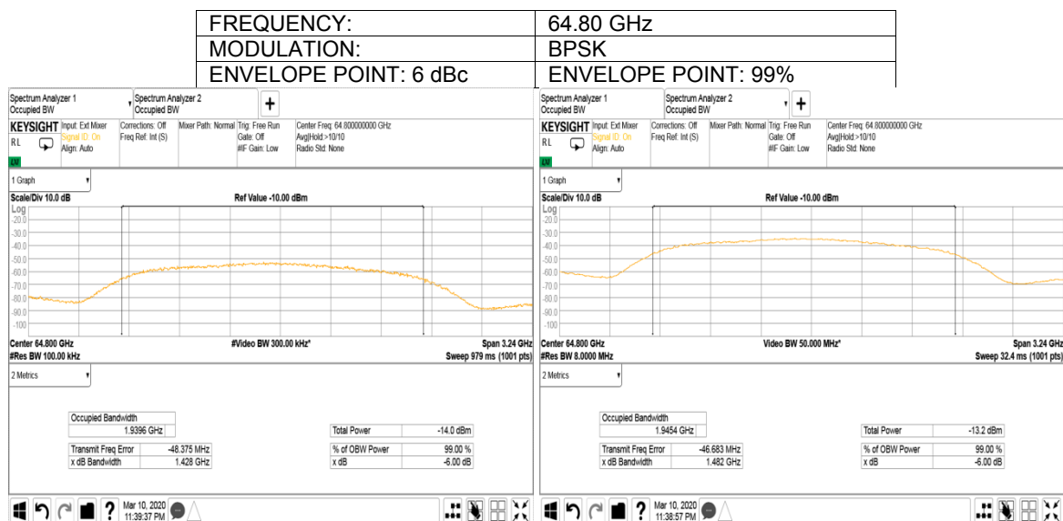
Plot 7.2.9 The 6dBc and 99% occupied bandwidth
