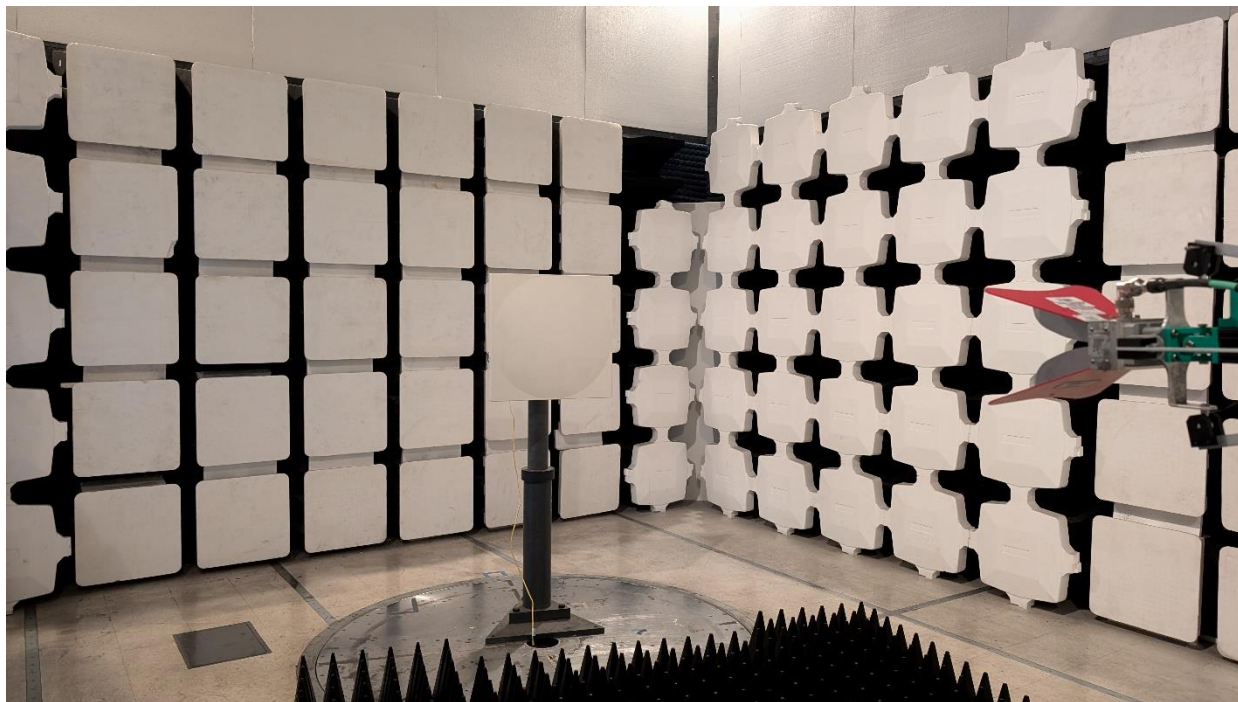
RW-9628-5872 Spurious Emissions 1-18GHz
