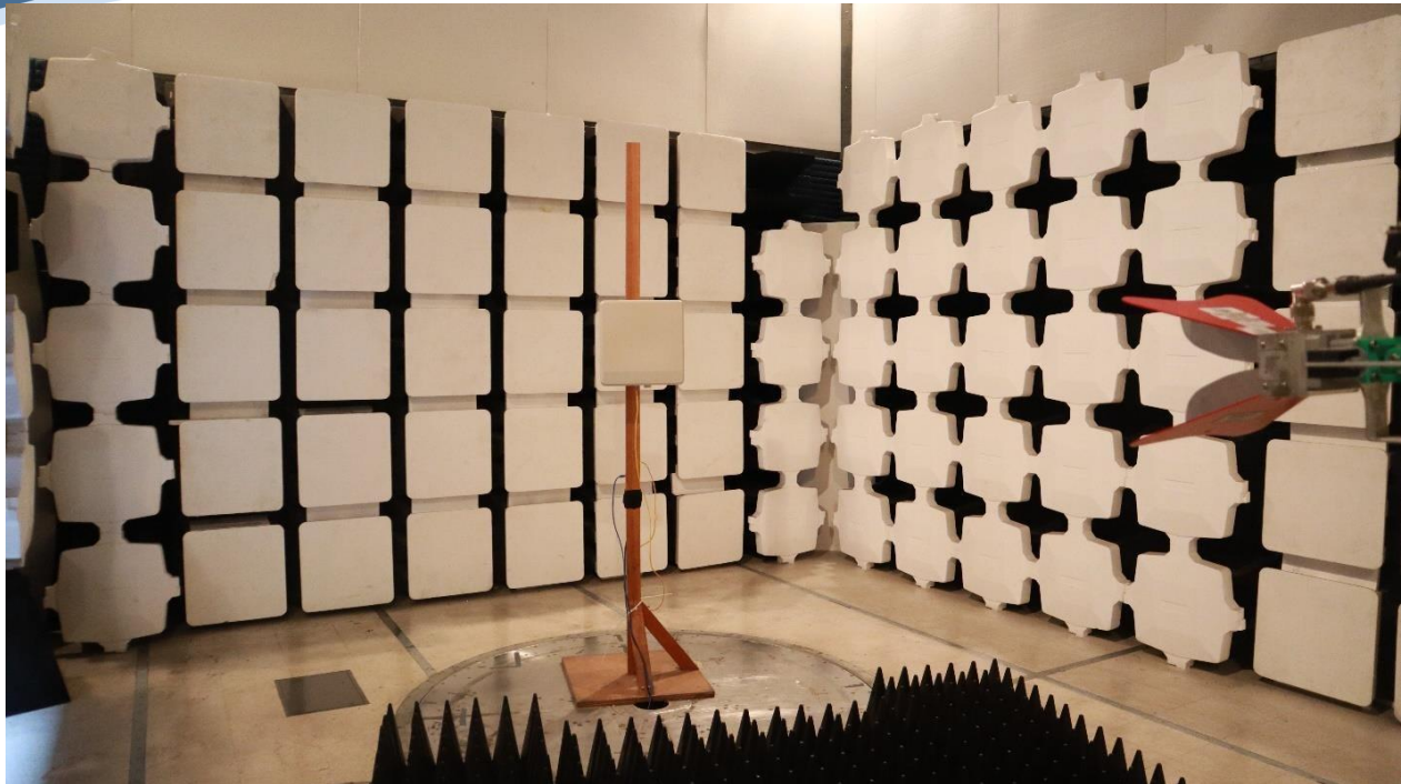
Spurious Emissions 1-18GHz AX6400
