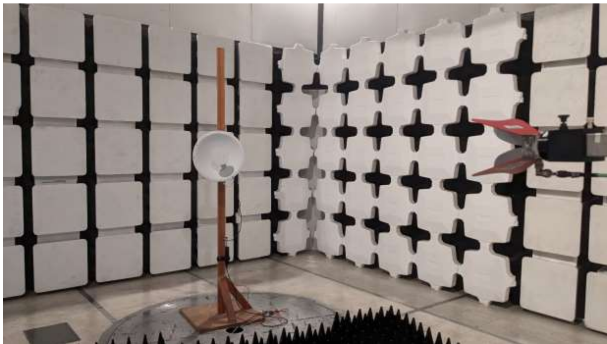
Spurious Emissions 25 dBi Dish
