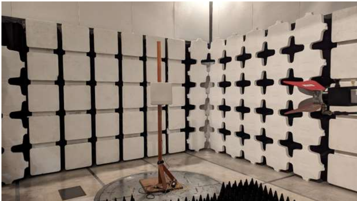
Spurious Emissions 24 dBi Panel
