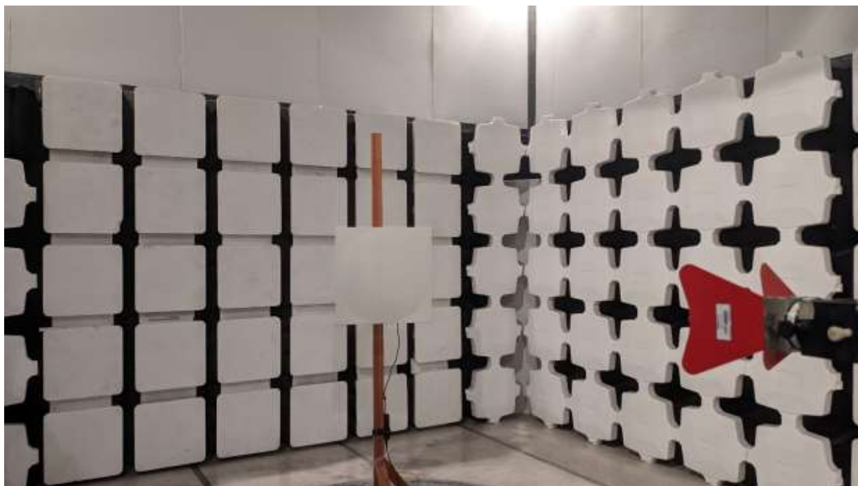
Spurious Emissions 28 dBi Directional
