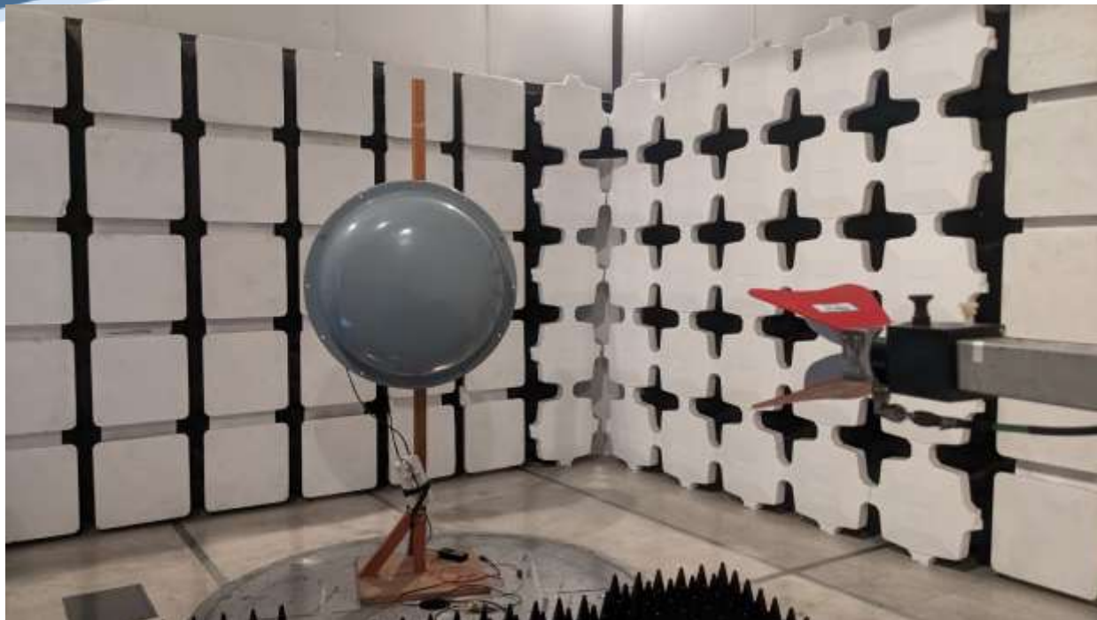
Spurious Emissions 32 dBi Dish
