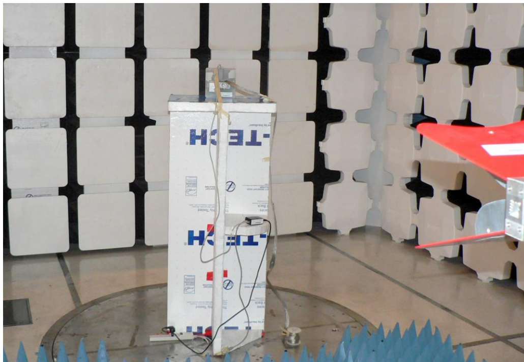
TX Spurious
