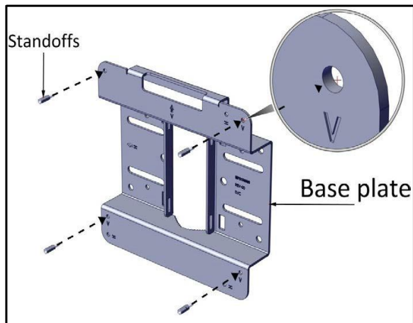
Figure 2-5: Fasten standoffs to base plate (for vertical pole)
