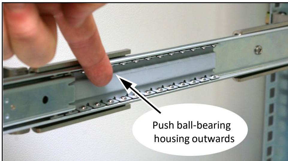
Figure 2-80: Inserting the drawer: Push ball-bearing housings outwards
