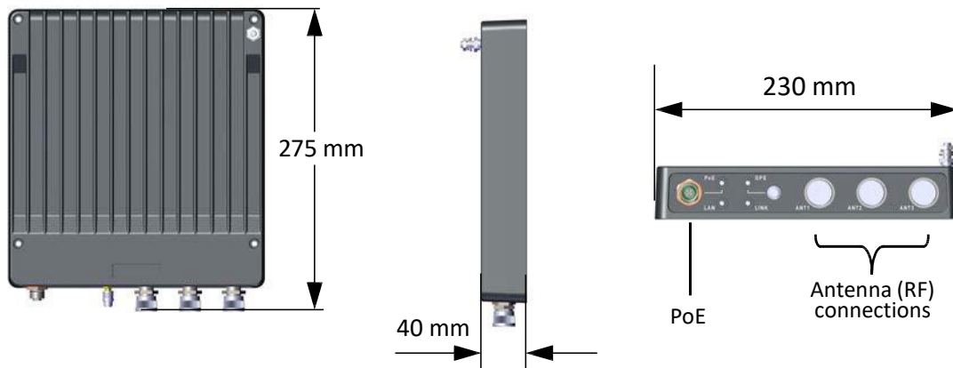
Figure 1-5: TMU radio
