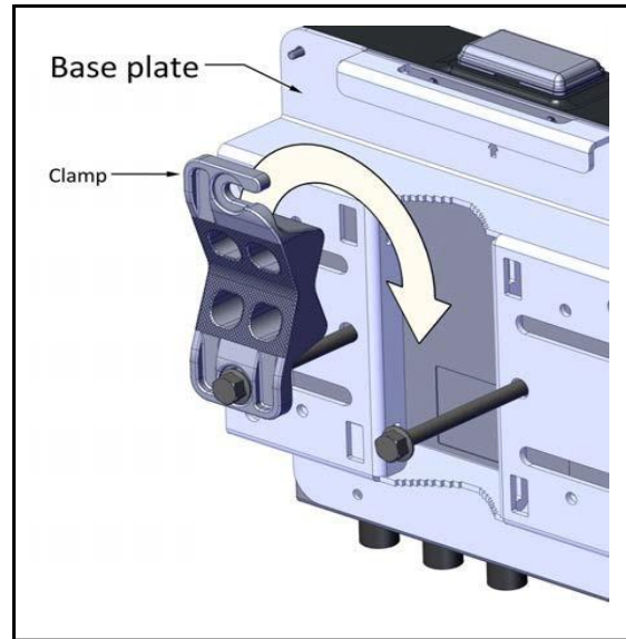
Figure 2-8: Thin pole: Do not completely tighten bolts
