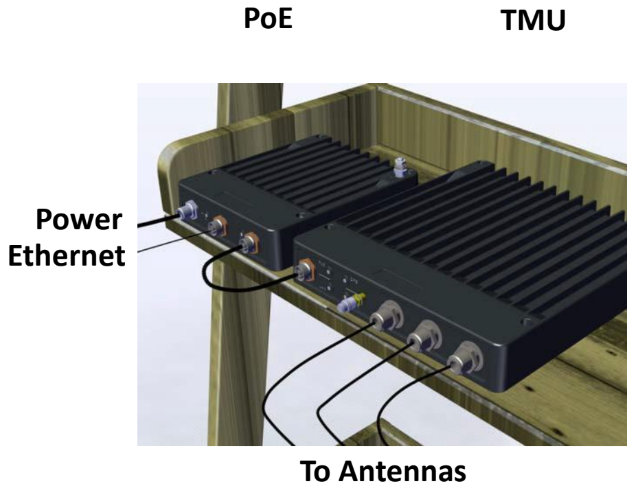
Figure 2-70: TMU mounted on a shelf
