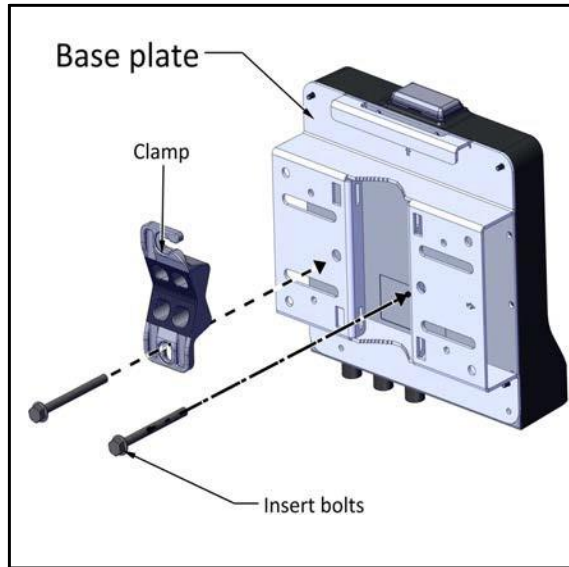
Figure 2-7: Thin pole: clamp to base plate
