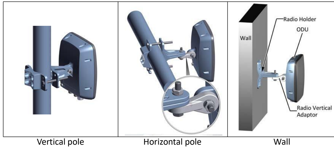
Figure 2-55: Mounted GSUs
