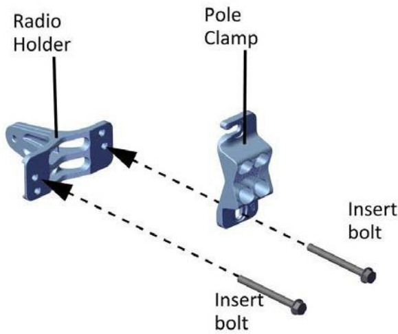
Figure 2-41: Connect Pole Clamp to Radio Holder
