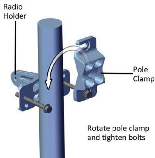
Figure 2-43: Rotate Clamp and tighten bolts
