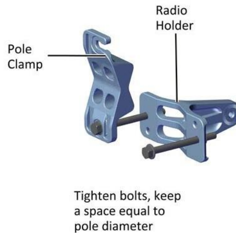
Figure 2-38: Tighten bolts
