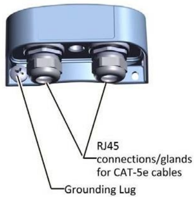
Figure 2-60: LPU: Bottom View
