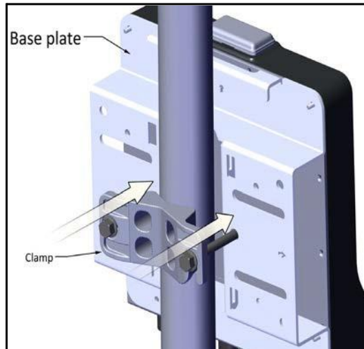
Figure 2-10: Thin pole: tighten bolt
